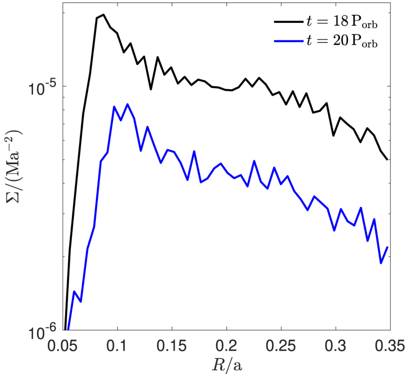
Figure 3. from Sustained Kozai–Lidov Oscillations in Misaligned Circumstellar Gas Disks null 2021 APJL 907 L14 doi:10.3847/2041-8213/abd4d6 https://dx.doi.org/10.3847/2041-8213/abd4d6 © 2021. The American Astronomical Society. All rights reserved.
