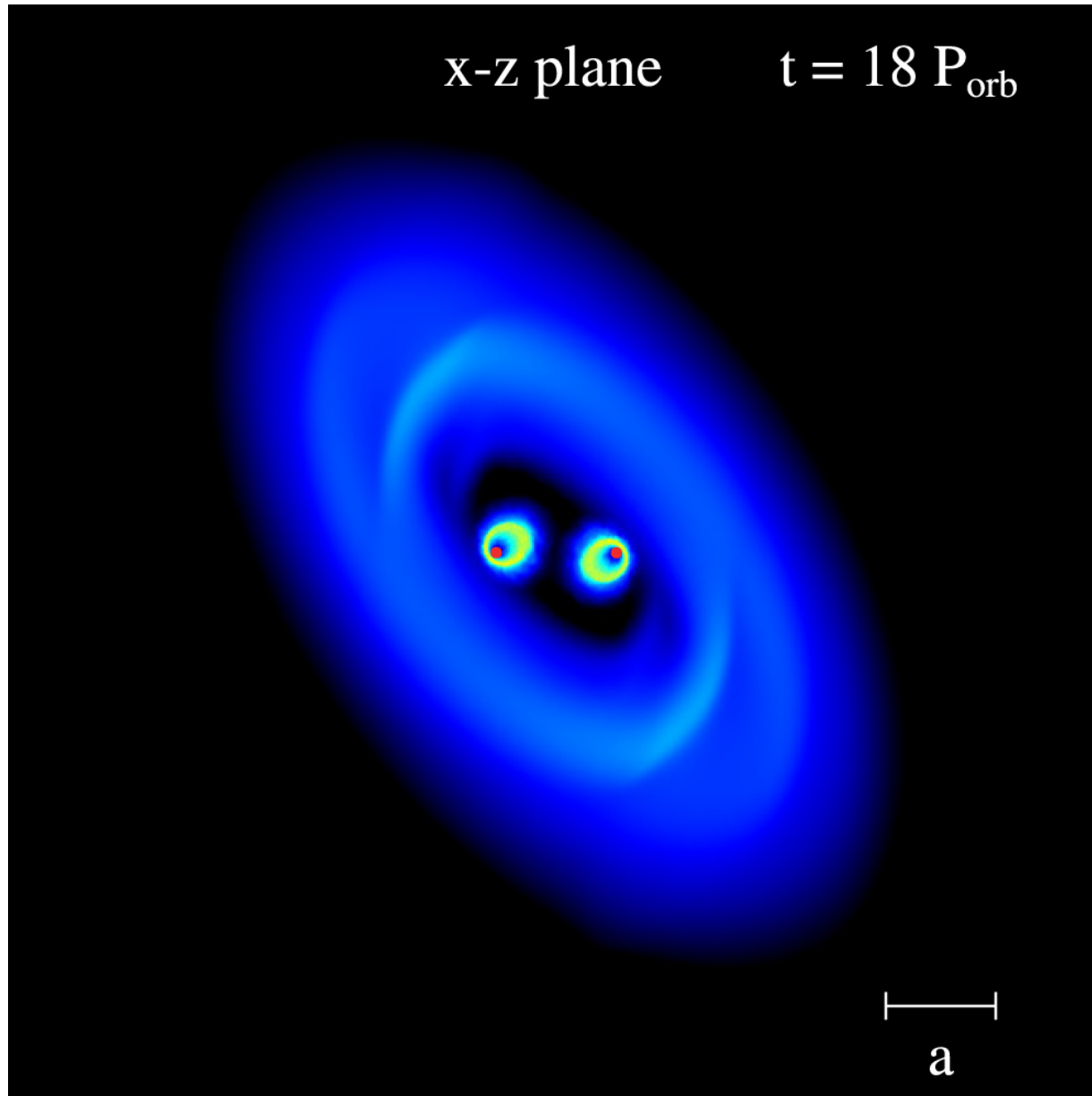
Figure 1. from Sustained Kozai–Lidov Oscillations in Misaligned Circumstellar Gas Disks null 2021 APJL 907 L14 doi:10.3847/2041-8213/abd4d6 https://dx.doi.org/10.3847/2041-8213/abd4d6 © 2021. The American Astronomical Society. All rights reserved.
