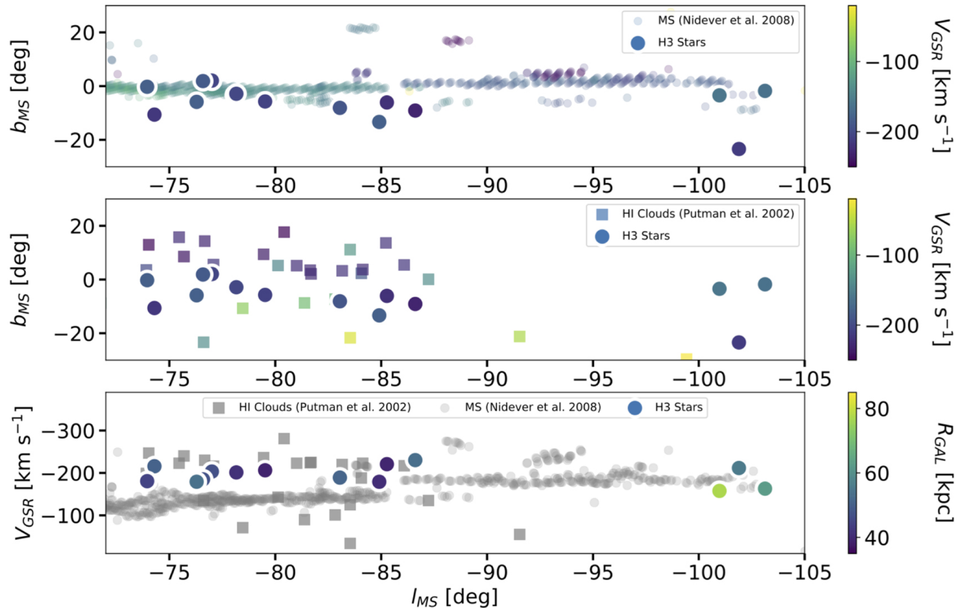
Figure 3. from Discovery of Magellanic Stellar Debris in the H3 Survey null 2020 APJL 905 L3 doi:10.3847/2041-8213/abcb83 https://dx.doi.org/10.3847/2041-8213/abcb83 © 2020. The American Astronomical Society. All rights reserved.
