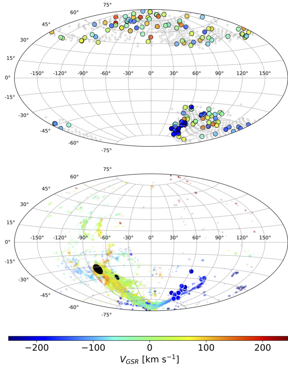
Figure 1. from Discovery of Magellanic Stellar Debris in the H3 Survey null 2020 APJL 905 L3 doi:10.3847/2041-8213/abcb83 https://dx.doi.org/10.3847/2041-8213/abcb83 © 2020. The American Astronomical Society. All rights reserved.
