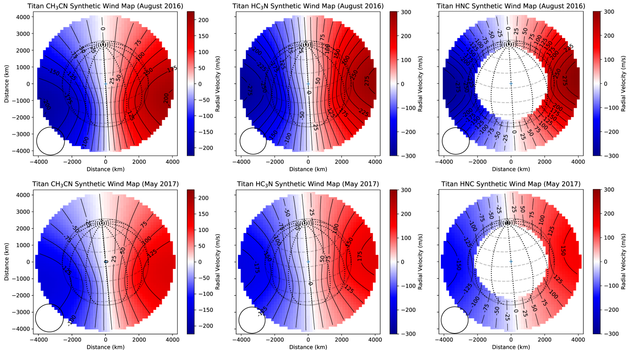
Figure 6. from Detection of Dynamical Instability in Titan's Thermospheric Jet null 2020 APJL 904 L12 doi:10.3847/2041-8213/abc688 https://dx.doi.org/10.3847/2041-8213/abc688
