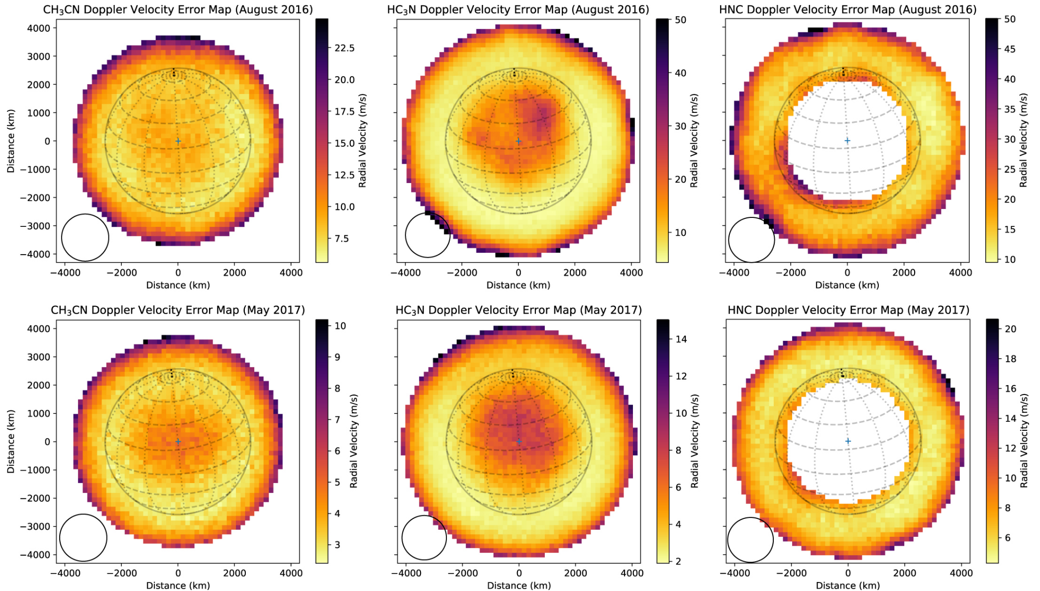
Figure 5. from Detection of Dynamical Instability in Titan's Thermospheric Jet null 2020 APJL 904 L12 doi:10.3847/2041-8213/abc688 https://dx.doi.org/10.3847/2041-8213/abc688
