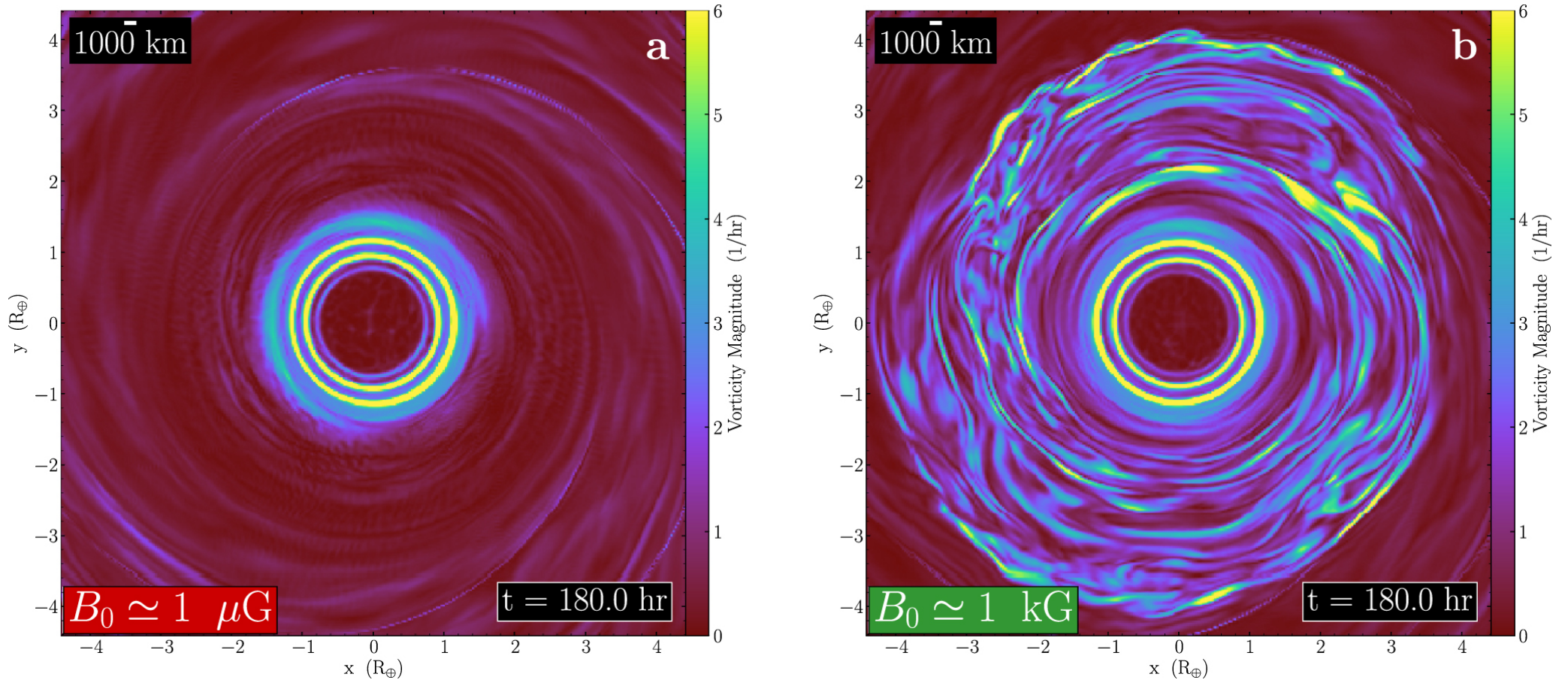
Figure 5. from A Magnetized, Moon-forming Giant Impact null 2020 APJL 903 L15 doi:10.3847/2041-8213/abbffd https://dx.doi.org/10.3847/2041-8213/abbffd © 2020. The American Astronomical Society. All rights reserved.
