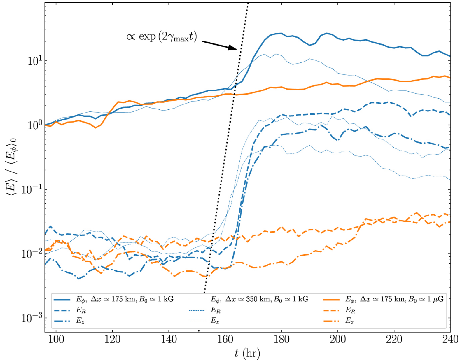
Figure 3. from A Magnetized, Moon-forming Giant Impact null 2020 APJL 903 L15 doi:10.3847/2041-8213/abbffd https://dx.doi.org/10.3847/2041-8213/abbffd © 2020. The American Astronomical Society. All rights reserved.
