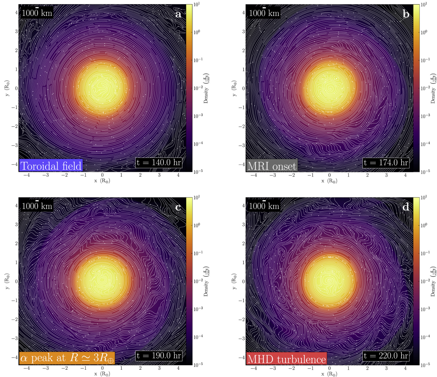
Figure 2. from A Magnetized, Moon-forming Giant Impact null 2020 APJL 903 L15 doi:10.3847/2041-8213/abbffd https://dx.doi.org/10.3847/2041-8213/abbffd © 2020. The American Astronomical Society. All rights reserved.
