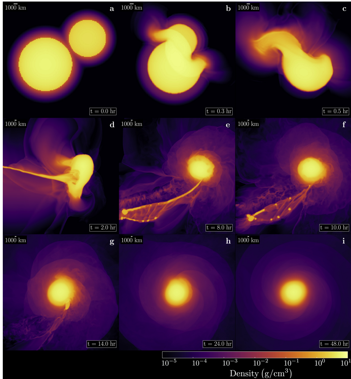
Figure 1. from A Magnetized, Moon-forming Giant Impact null 2020 APJL 903 L15 doi:10.3847/2041-8213/abbffd https://dx.doi.org/10.3847/2041-8213/abbffd © 2020. The American Astronomical Society. All rights reserved.
