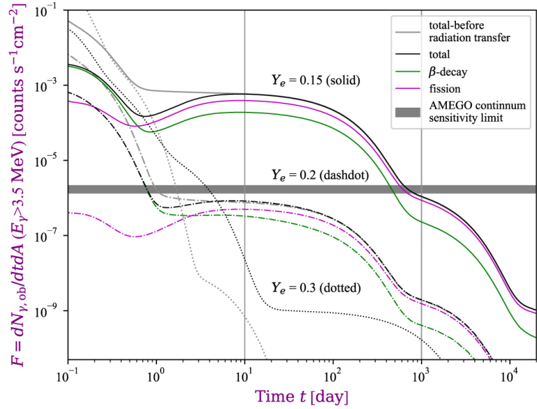
Figure 5. from MeV Gamma Rays from Fission: A Distinct Signature of Actinide Production in Neutron Star Mergers null 2020 APJL 903 L3 doi:10.3847/2041-8213/abbe18 https://dx.doi.org/10.3847/2041-8213/abbe18 © 2020. The American Astronomical Society. All rights reserved.
