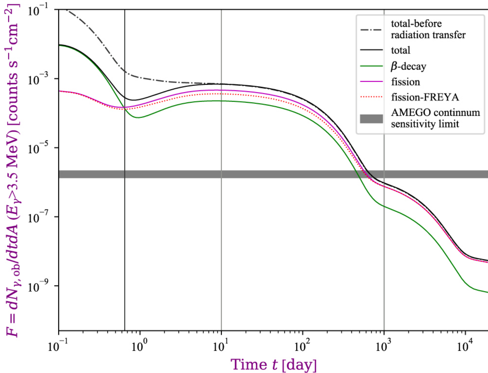
Figure 4. from MeV Gamma Rays from Fission: A Distinct Signature of Actinide Production in Neutron Star Mergers null 2020 APJL 903 L3 doi:10.3847/2041-8213/abbe18 https://dx.doi.org/10.3847/2041-8213/abbe18 © 2020. The American Astronomical Society. All rights reserved.
