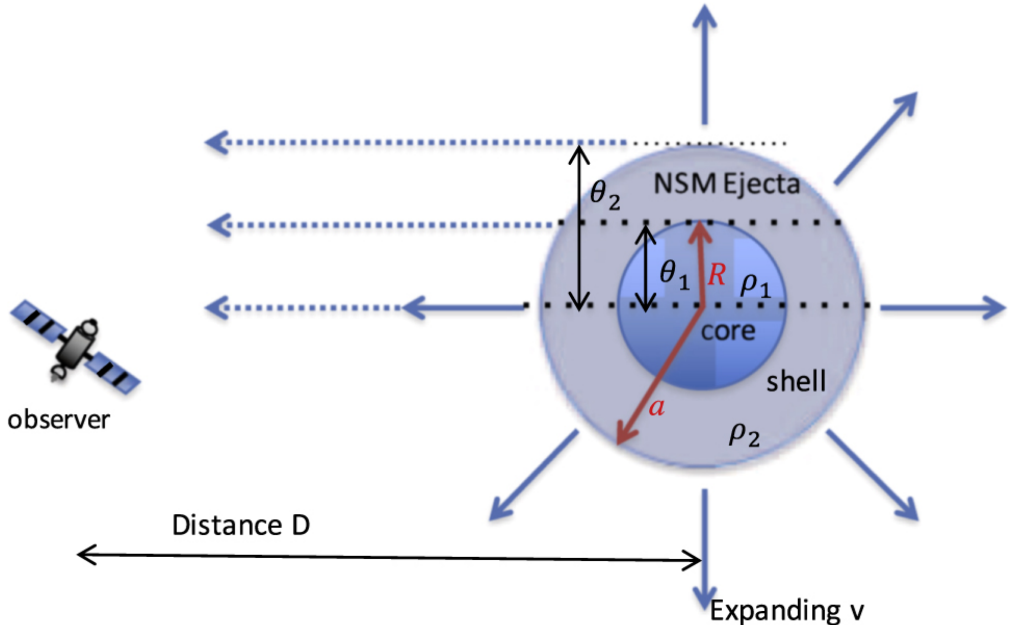
Figure 2. from MeV Gamma Rays from Fission: A Distinct Signature of Actinide Production in Neutron Star Mergers null 2020 APJL 903 L3 doi:10.3847/2041-8213/abbe18 https://dx.doi.org/10.3847/2041-8213/abbe18 © 2020. The American Astronomical Society. All rights reserved.
