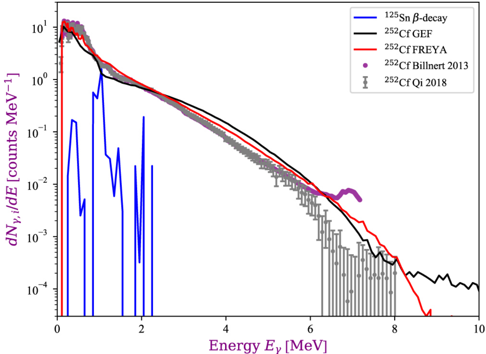
Figure 1. from MeV Gamma Rays from Fission: A Distinct Signature of Actinide Production in Neutron Star Mergers null 2020 APJL 903 L3 doi:10.3847/2041-8213/abbe18 https://dx.doi.org/10.3847/2041-8213/abbe18 © 2020. The American Astronomical Society. All rights reserved.
