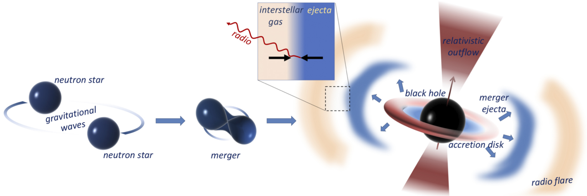
Figure 1. from FIRST J1419+3940 as the First Observed Radio Flare from a Neutron Star Merger null 2020 APJL 902 L23 doi:10.3847/2041-8213/abbb8a https://dx.doi.org/10.3847/2041-8213/abbb8a © 2020. The American Astronomical Society. All rights reserved.
