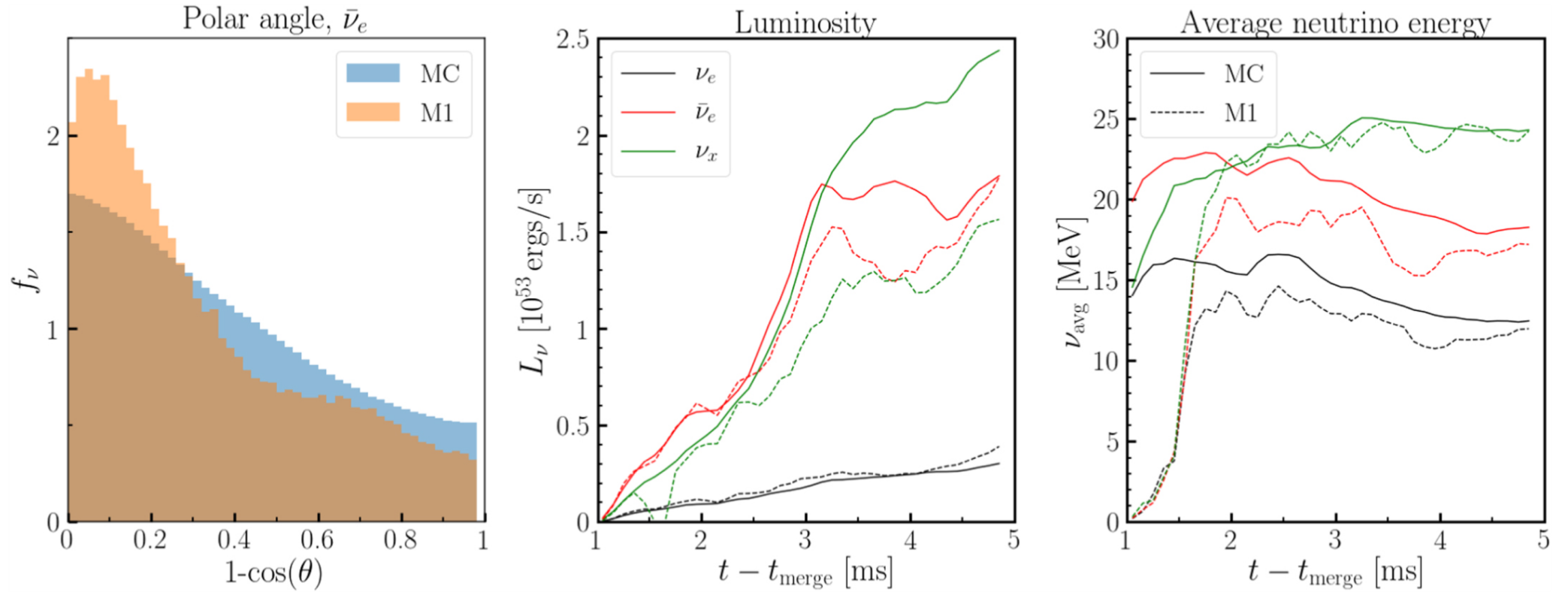
Figure 5. from Monte-Carlo Neutrino Transport in Neutron Star Merger Simulations null 2020 APJL 902 L27 doi:10.3847/2041-8213/abbb87 https://dx.doi.org/10.3847/2041-8213/abbb87 © 2020. The American Astronomical Society. All rights reserved.
