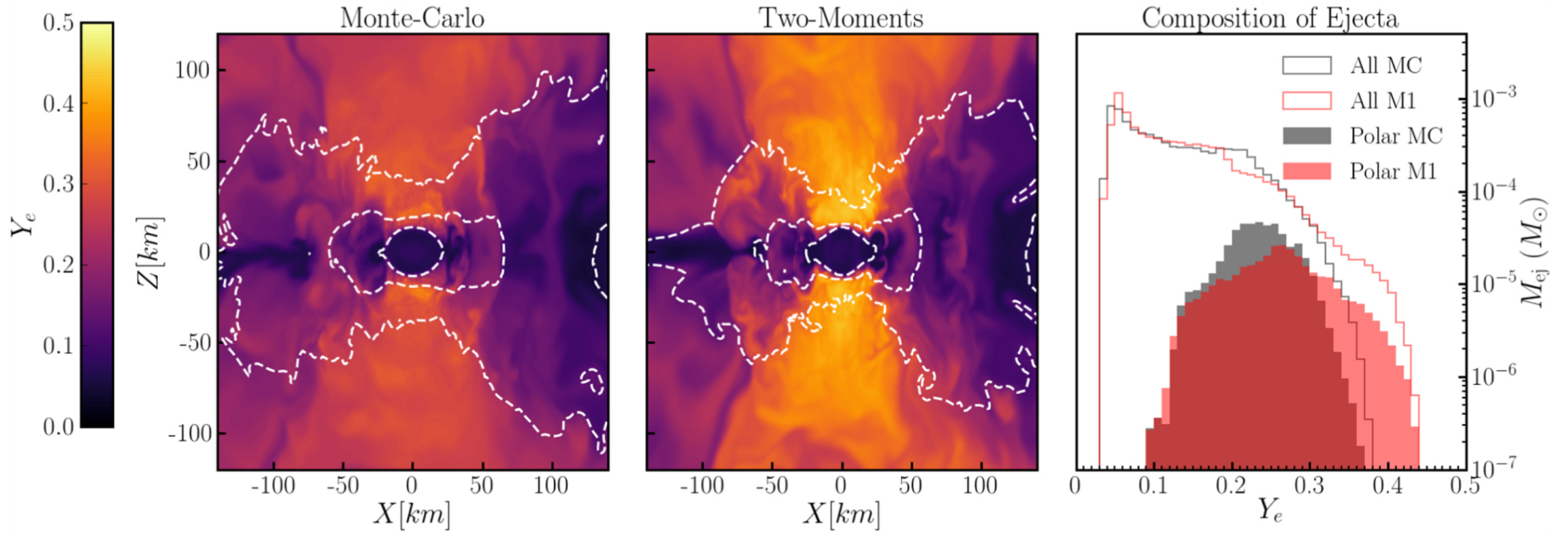
Figure 3. from Monte-Carlo Neutrino Transport in Neutron Star Merger Simulations null 2020 APJL 902 L27 doi:10.3847/2041-8213/abbb87 https://dx.doi.org/10.3847/2041-8213/abbb87 © 2020. The American Astronomical Society. All rights reserved.
