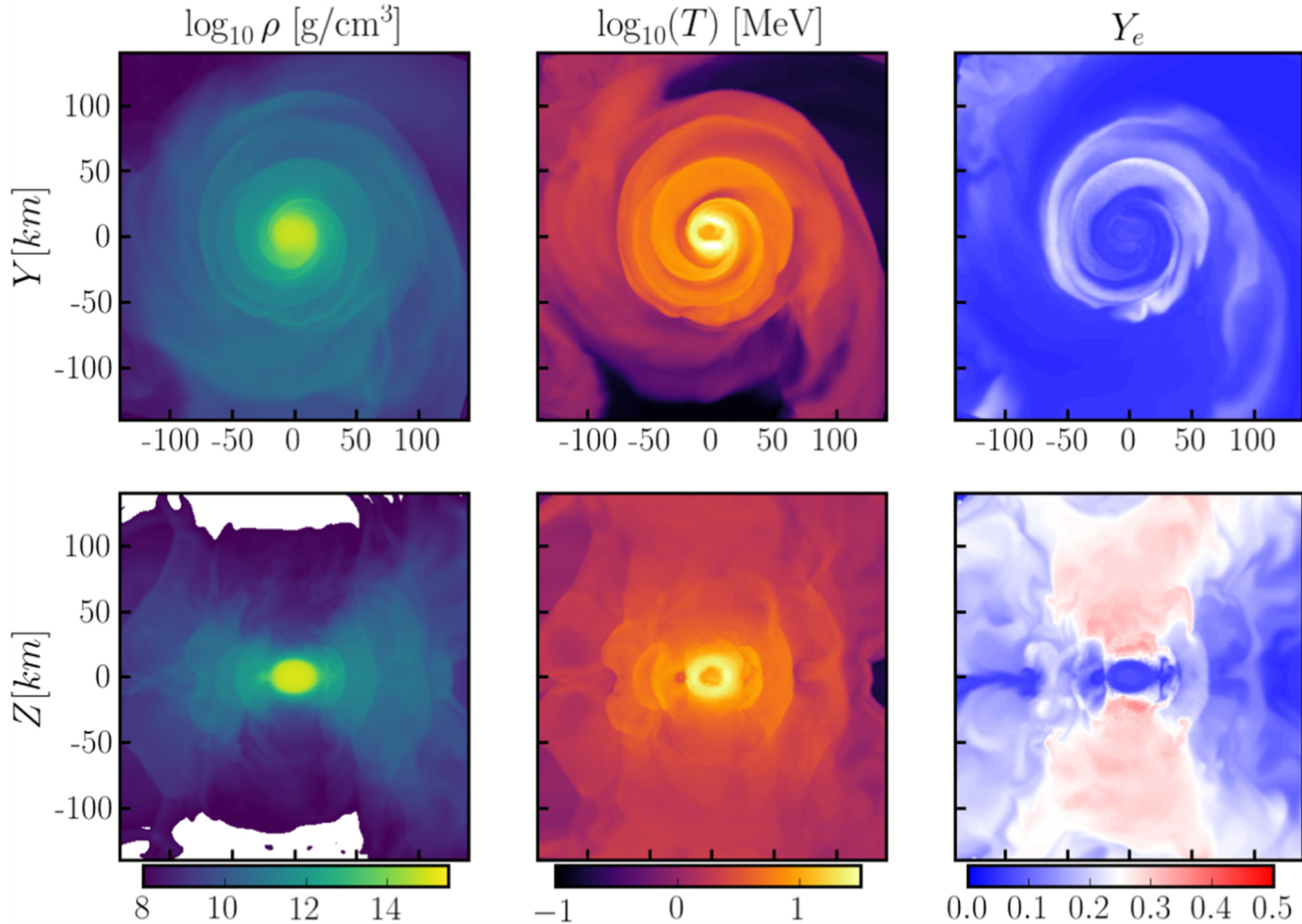
Figure 2. from Monte-Carlo Neutrino Transport in Neutron Star Merger Simulations null 2020 APJL 902 L27 doi:10.3847/2041-8213/abbb87 https://dx.doi.org/10.3847/2041-8213/abbb87 © 2020. The American Astronomical Society. All rights reserved.
