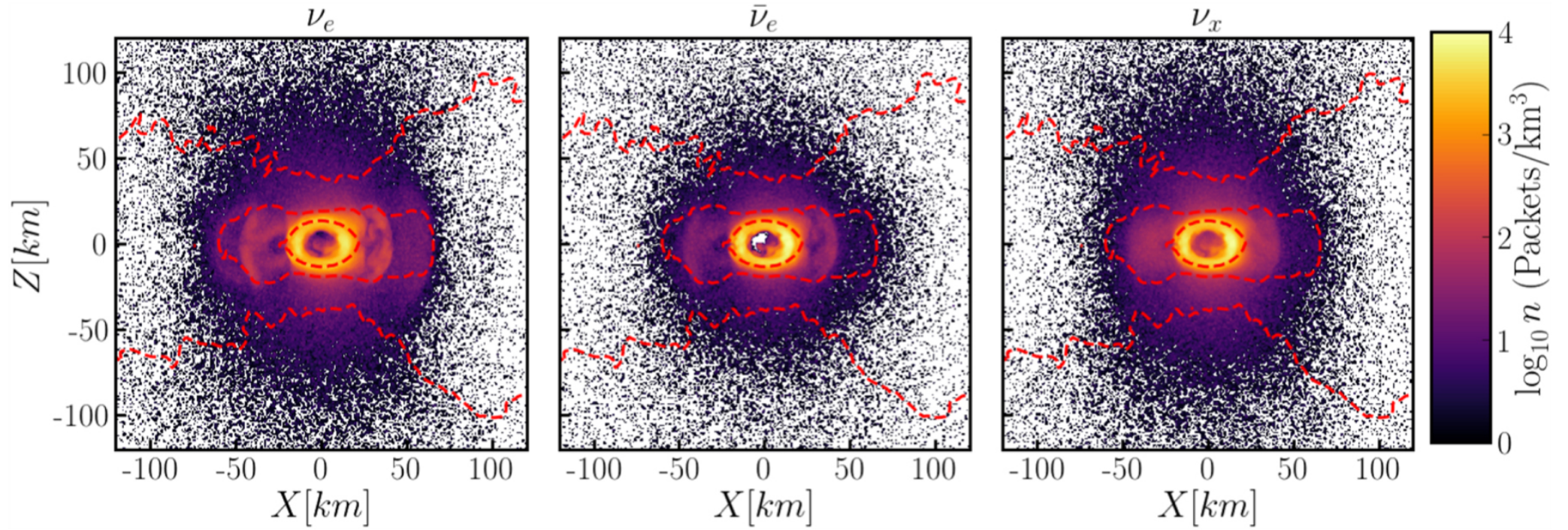
Figure 1. from Monte-Carlo Neutrino Transport in Neutron Star Merger Simulations null 2020 APJL 902 L27 doi:10.3847/2041-8213/abbb87 https://dx.doi.org/10.3847/2041-8213/abbb87 © 2020. The American Astronomical Society. All rights reserved.
