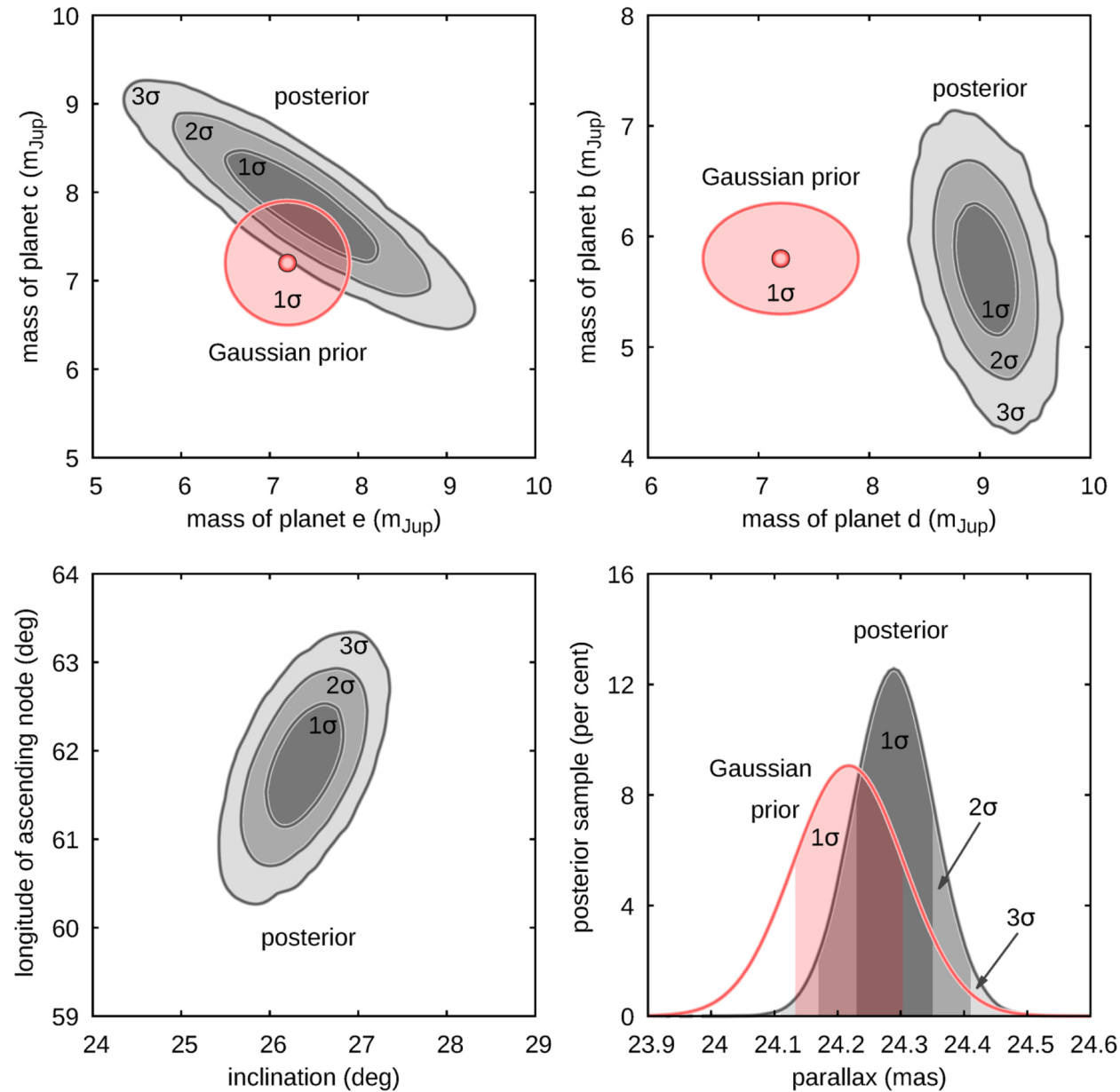
Figure 3. from An Exact, Generalized Laplace Resonance in the HR 8799 Planetary System null 2020 APJL 902 L40 doi:10.3847/2041-8213/abb881 https://dx.doi.org/10.3847/2041-8213/abb881 © 2020. The American Astronomical Society. All rights reserved.
