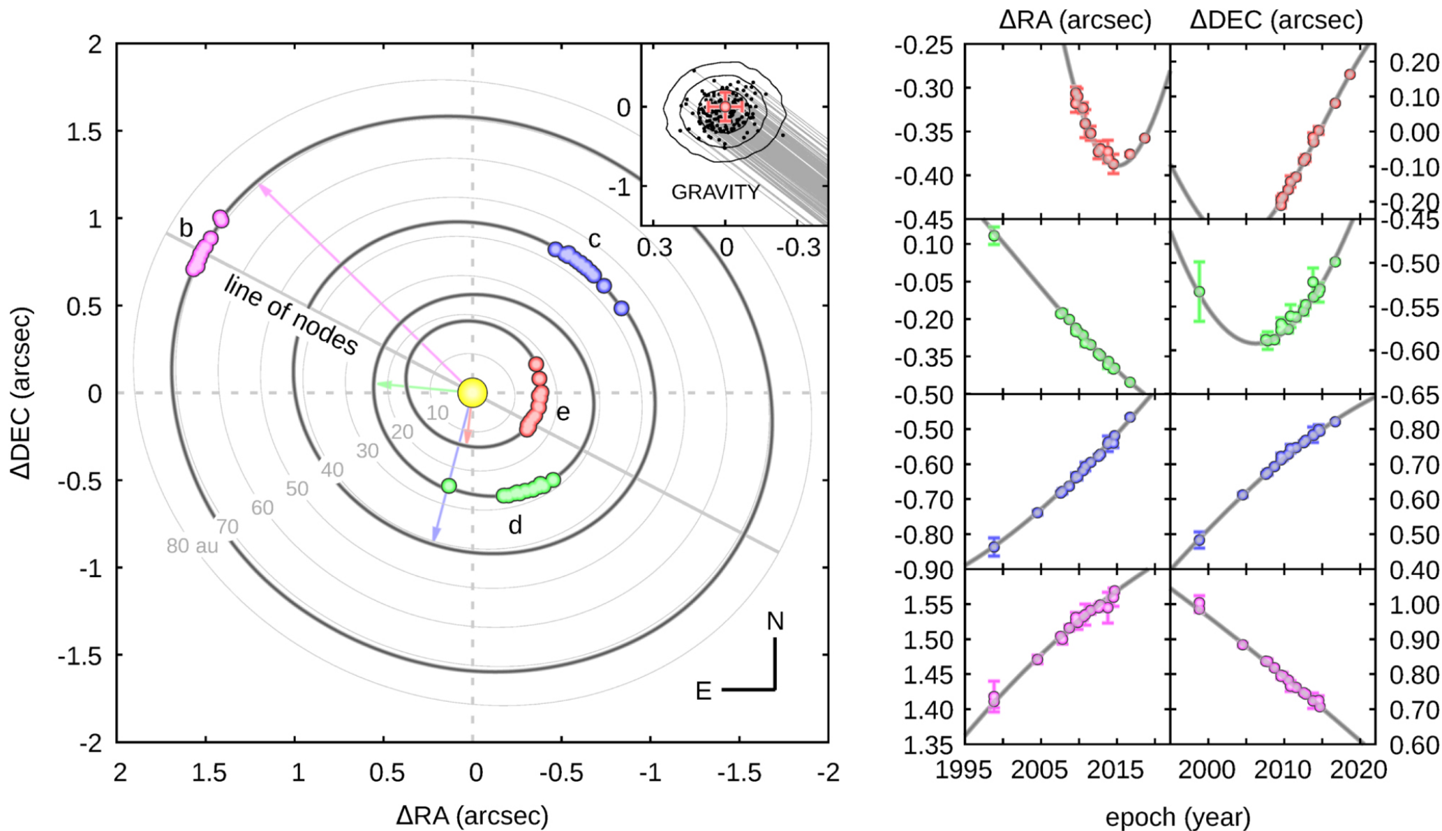
Figure 1. from An Exact, Generalized Laplace Resonance in the HR 8799 Planetary System null 2020 APJL 902 L40 doi:10.3847/2041-8213/abb881 https://dx.doi.org/10.3847/2041-8213/abb881 © 2020. The American Astronomical Society. All rights reserved.
