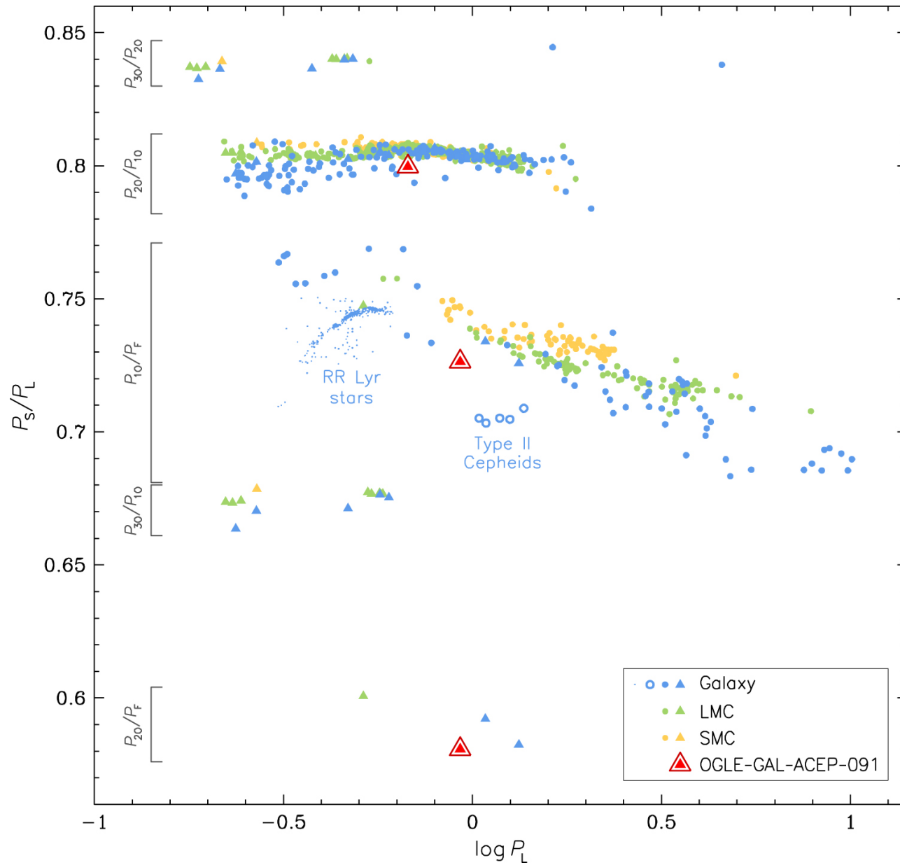
Figure 2. from OGLE-GAL-ACEP-091: The First Known Multi-mode Anomalous Cepheid null 2020 APJL 901 L25 doi:10.3847/2041-8213/abb817 https://dx.doi.org/10.3847/2041-8213/abb817 © 2020. The American Astronomical Society. All rights reserved.
