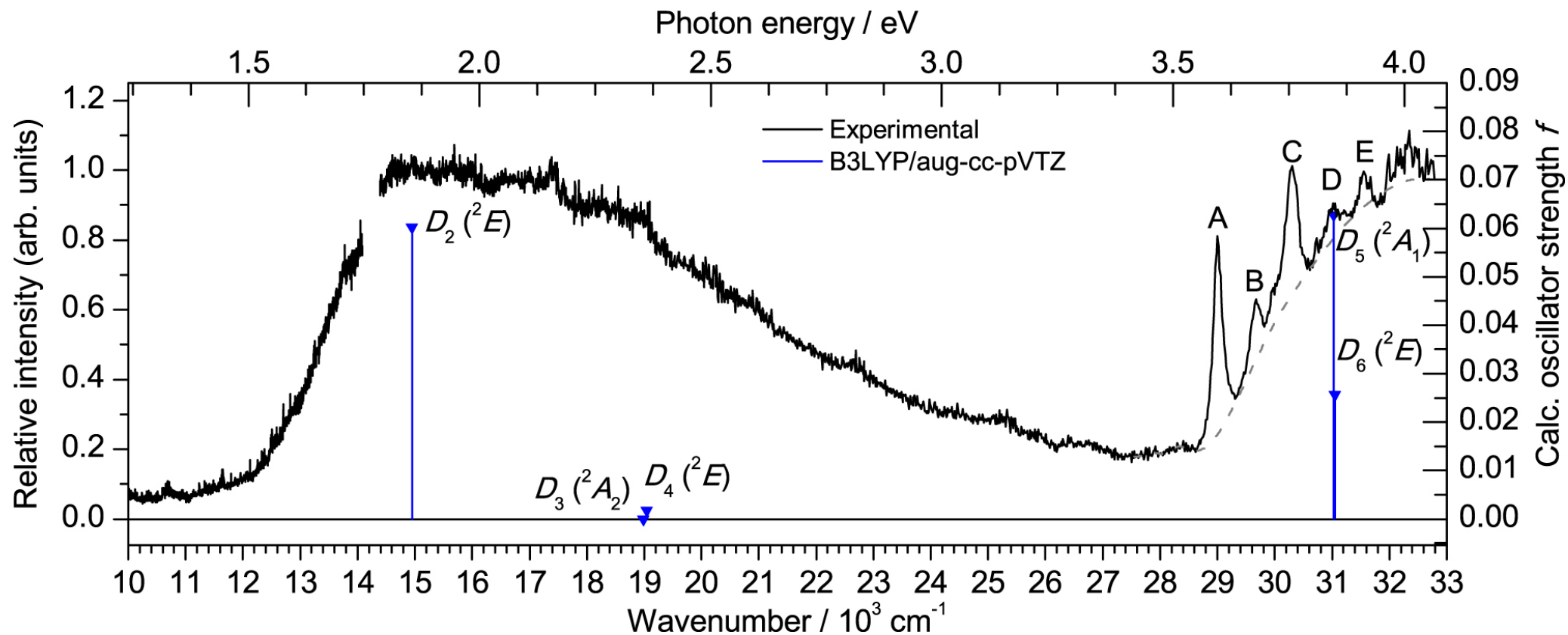
Figure 3. from Optical Spectrum of the Adamantane Radical Cation null 2020 APJL 900 L20 doi:10.3847/2041-8213/abafbd https://dx.doi.org/10.3847/2041-8213/abafbd © 2020. The American Astronomical Society. All rights reserved.
