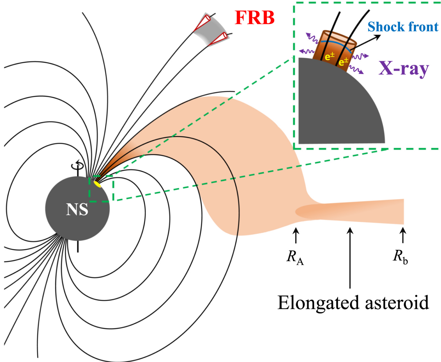
Figure 1. from FRB 200428: An Impact between an Asteroid and a Magnetar null 2020 APJL 898 L55 doi:10.3847/2041-8213/aba83c https://dx.doi.org/10.3847/2041-8213/aba83c © 2020. The American Astronomical Society. All rights reserved.
