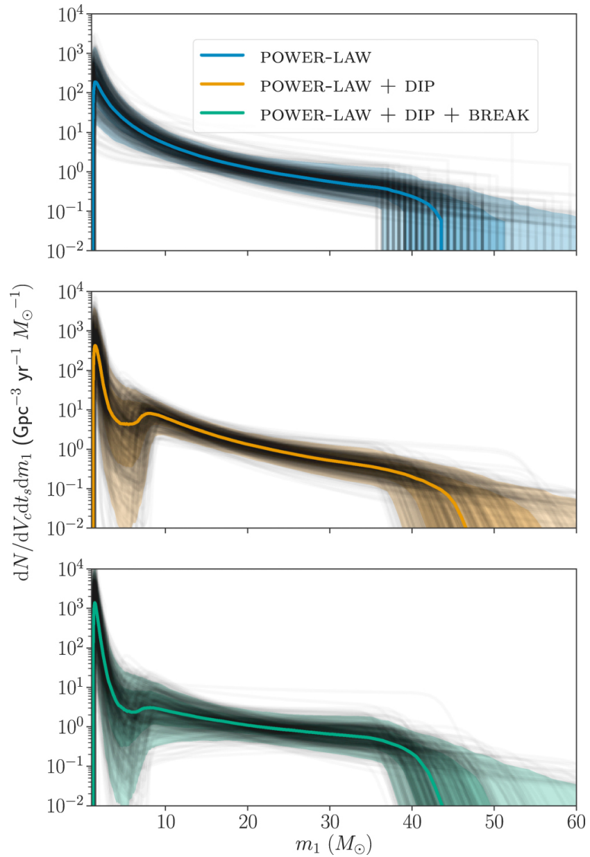
Figure 3. from Does Matter Matter? Using the Mass Distribution to Distinguish Neutron Stars and Black Holes null 2020 APJL 899 L8 doi:10.3847/2041-8213/aba7b6 https://dx.doi.org/10.3847/2041-8213/aba7b6
