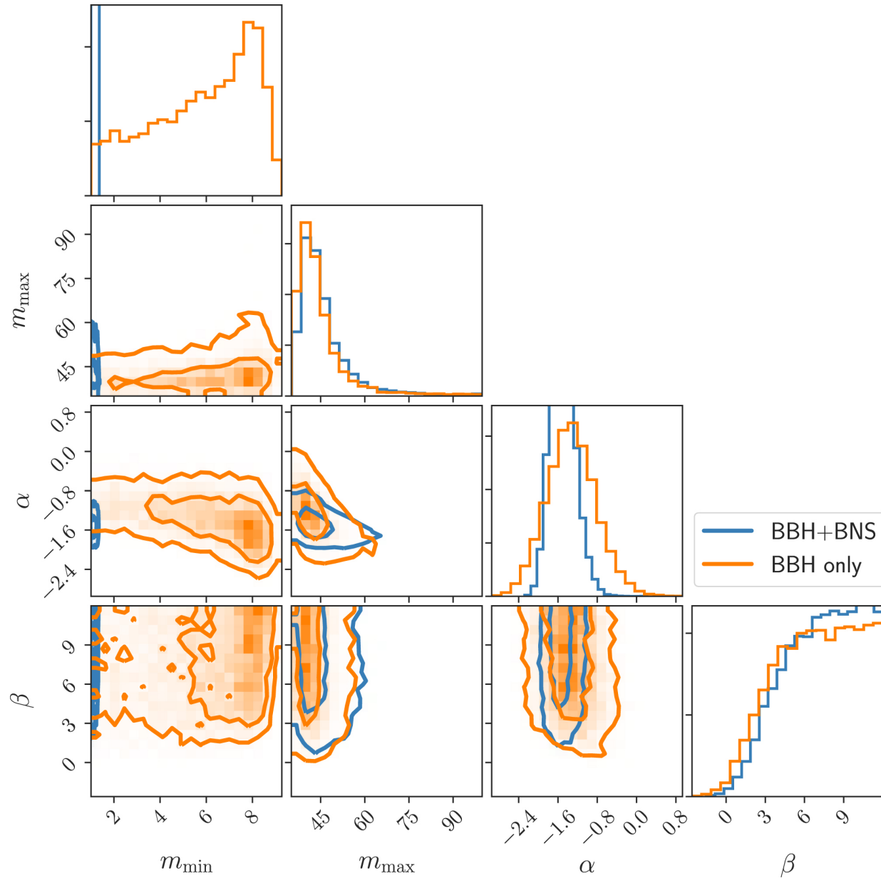
Figure 2. from Does Matter Matter? Using the Mass Distribution to Distinguish Neutron Stars and Black Holes null 2020 APJL 899 L8 doi:10.3847/2041-8213/aba7b6 https://dx.doi.org/10.3847/2041-8213/aba7b6 © 2020. The American Astronomical Society. All rights reserved.
