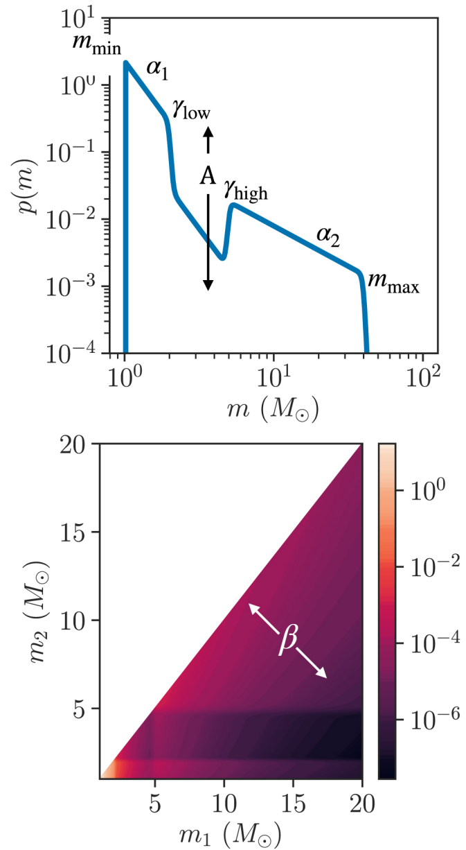
Figure 1. from Does Matter Matter? Using the Mass Distribution to Distinguish Neutron Stars and Black Holes null 2020 APJL 899 L8 doi:10.3847/2041-8213/aba7b6 https://dx.doi.org/10.3847/2041-8213/aba7b6 © 2020. The American Astronomical Society. All rights reserved.
