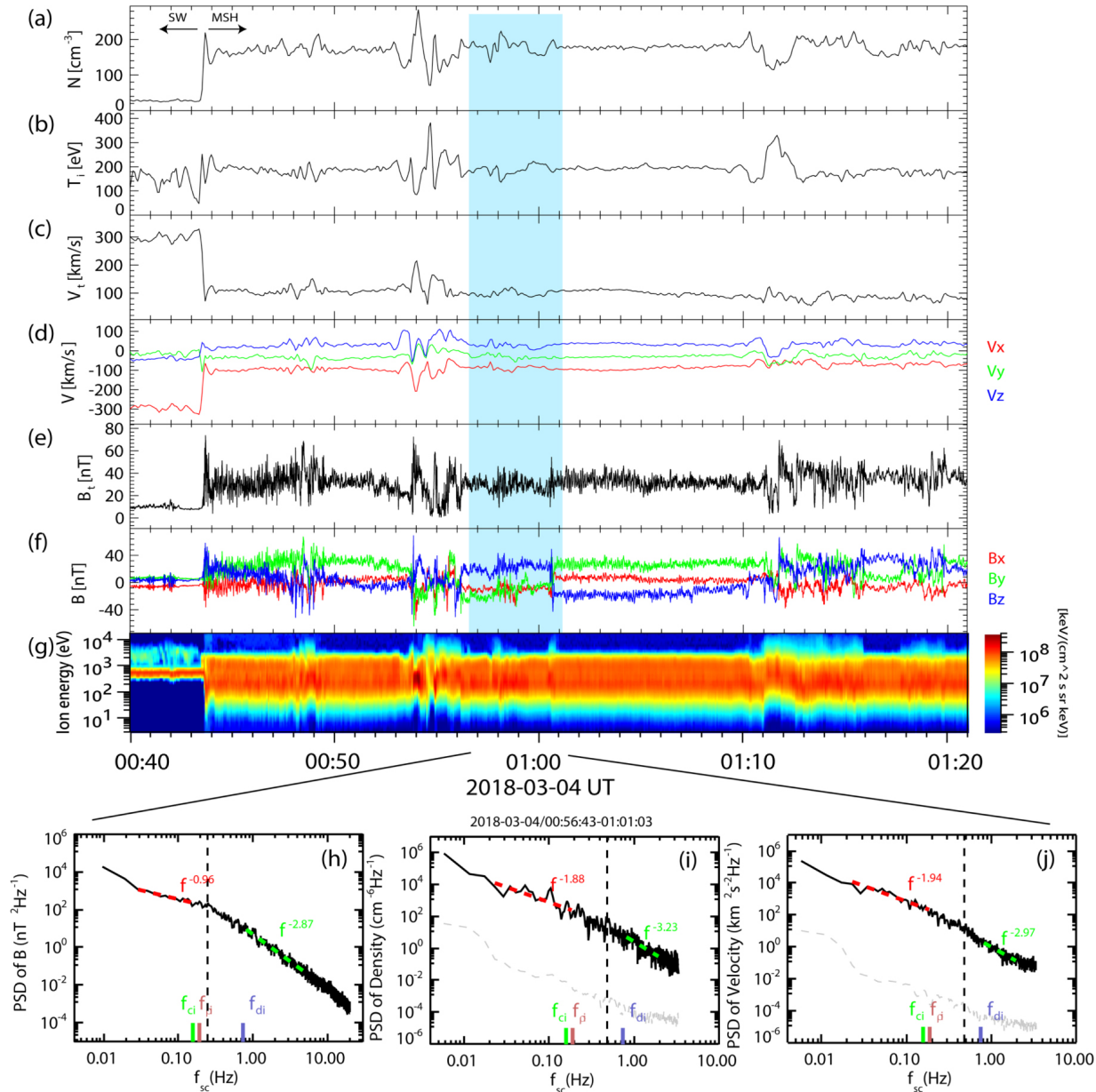
Figure 1. from Evolution of the Earth's Magnetosheath Turbulence: A Statistical Study Based on MMS Observations null 2020 APJL 898 L43 doi:10.3847/2041-8213/aba531 https://dx.doi.org/10.3847/2041-8213/aba531
