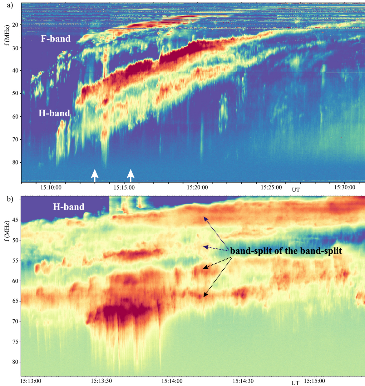
Figure 2. from Fine Structure of a Solar Type II Radio Burst Observed by LOFAR null 2020 APJL 897 L15 doi:10.3847/2041-8213/ab9abc https://dx.doi.org/10.3847/2041-8213/ab9abc © 2020. The American Astronomical Society. All rights reserved.
