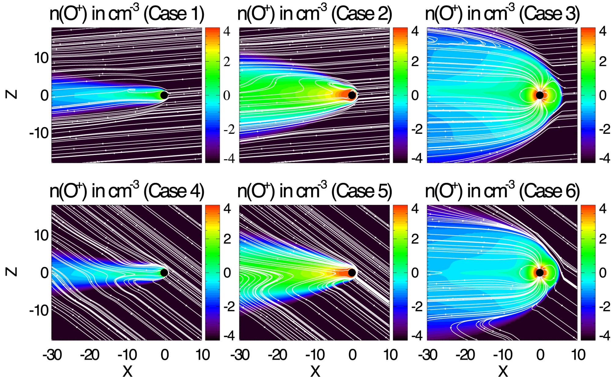
Figure 3. from Atmospheric Escape From TOI-700 d: Venus versus Earth Analogs null 2020 APJL 896 L24 doi:10.3847/2041-8213/ab982f https://dx.doi.org/10.3847/2041-8213/ab982f © 2020. The American Astronomical Society. All rights reserved.
