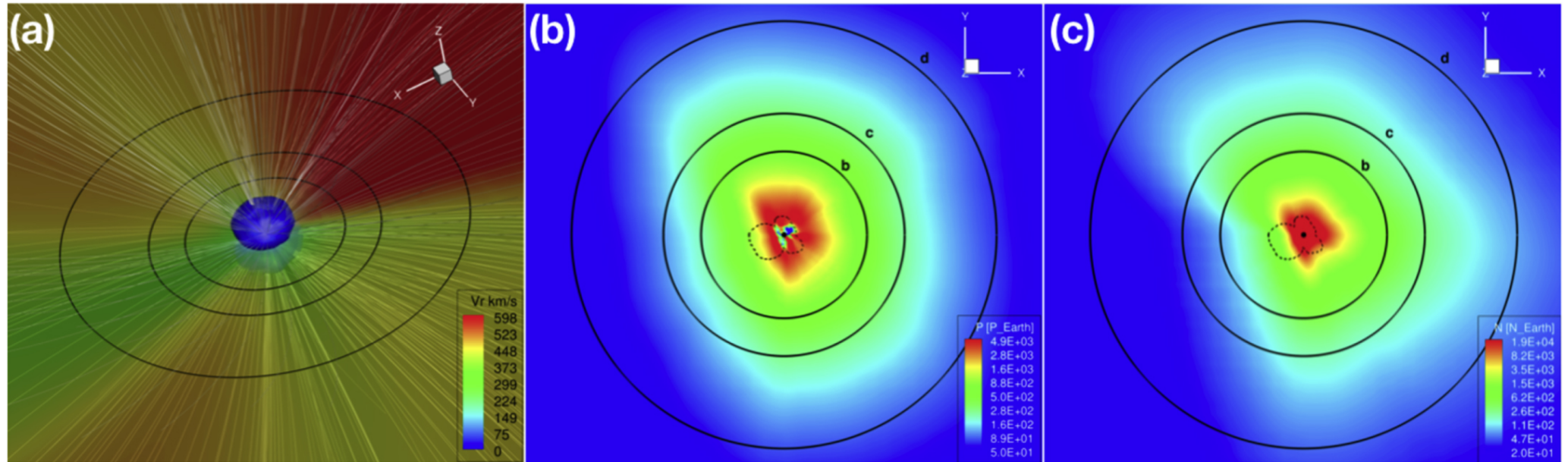
Figure 1. from Atmospheric Escape From TOI-700 d: Venus versus Earth Analogs null 2020 APJL 896 L24 doi:10.3847/2041-8213/ab982f https://dx.doi.org/10.3847/2041-8213/ab982f © 2020. The American Astronomical Society. All rights reserved.
