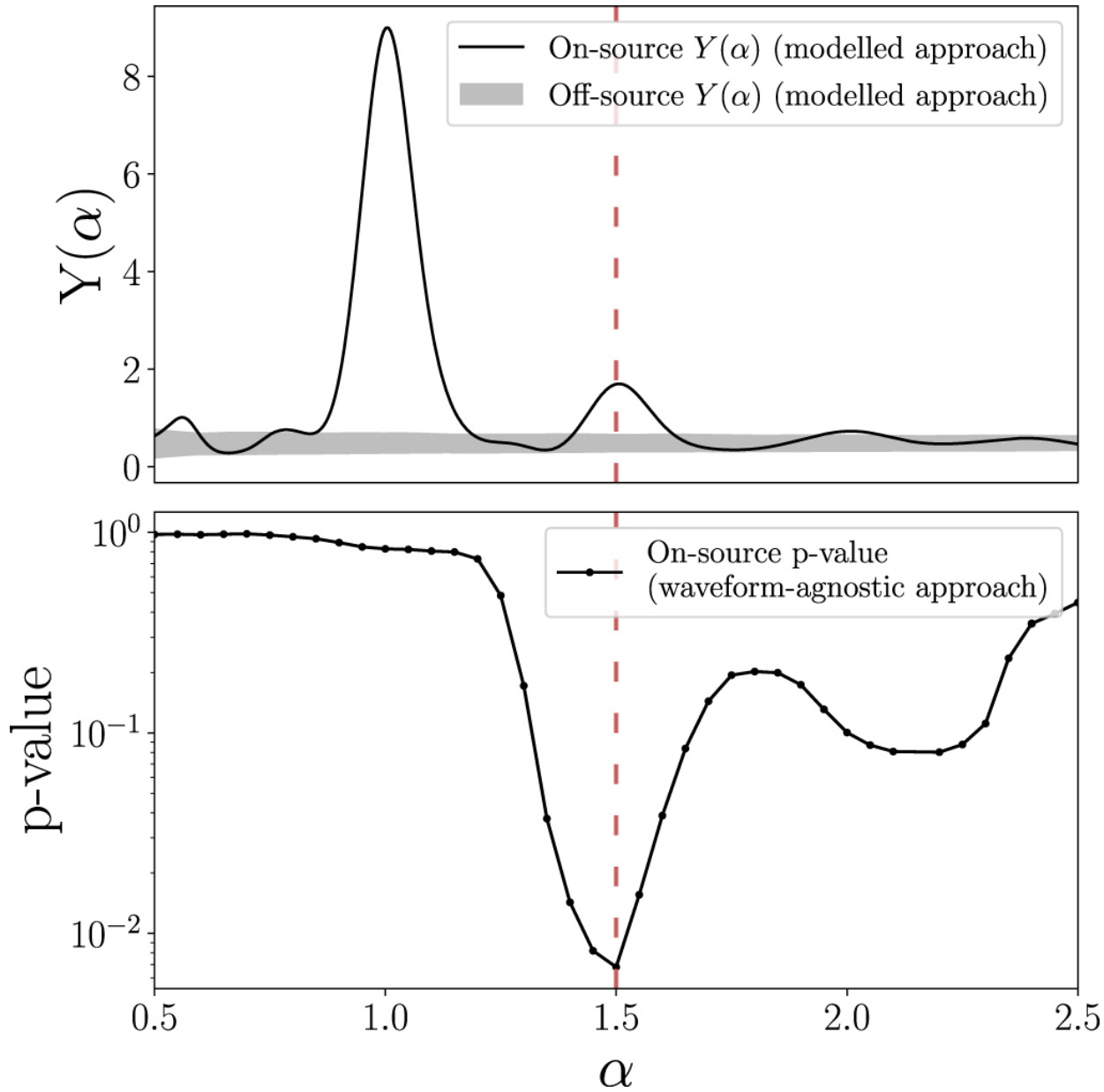
Figure 7. from GW190814: Gravitational Waves from the Coalescence of a 23 Solar Mass Black Hole with a 2.6 Solar Mass Compact Object null 2020 APJL 896 L44 doi:10.3847/2041-8213/ab960f https://dx.doi.org/10.3847/2041-8213/ab960f © 2020. The American Astronomical Society.
