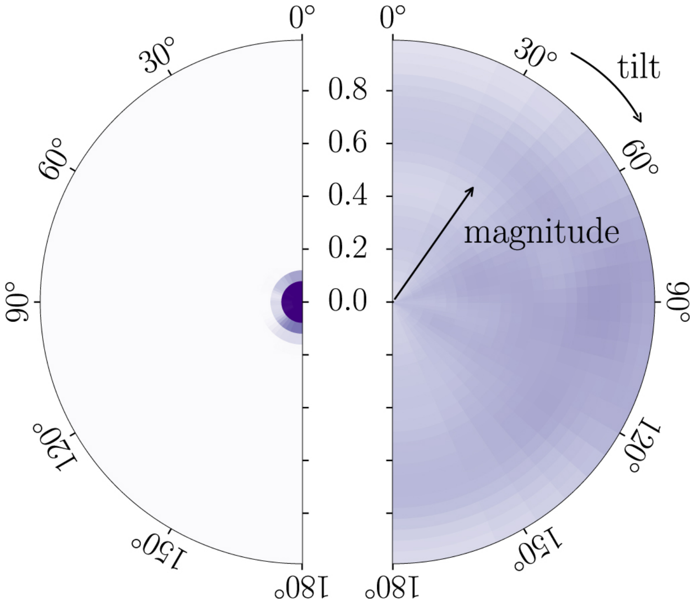
Figure 6. from GW190814: Gravitational Waves from the Coalescence of a 23 Solar Mass Black Hole with a 2.6 Solar Mass Compact Object null 2020 APJL 896 L44 doi:10.3847/2041-8213/ab960f https://dx.doi.org/10.3847/2041-8213/ab960f © 2020. The American Astronomical Society.
