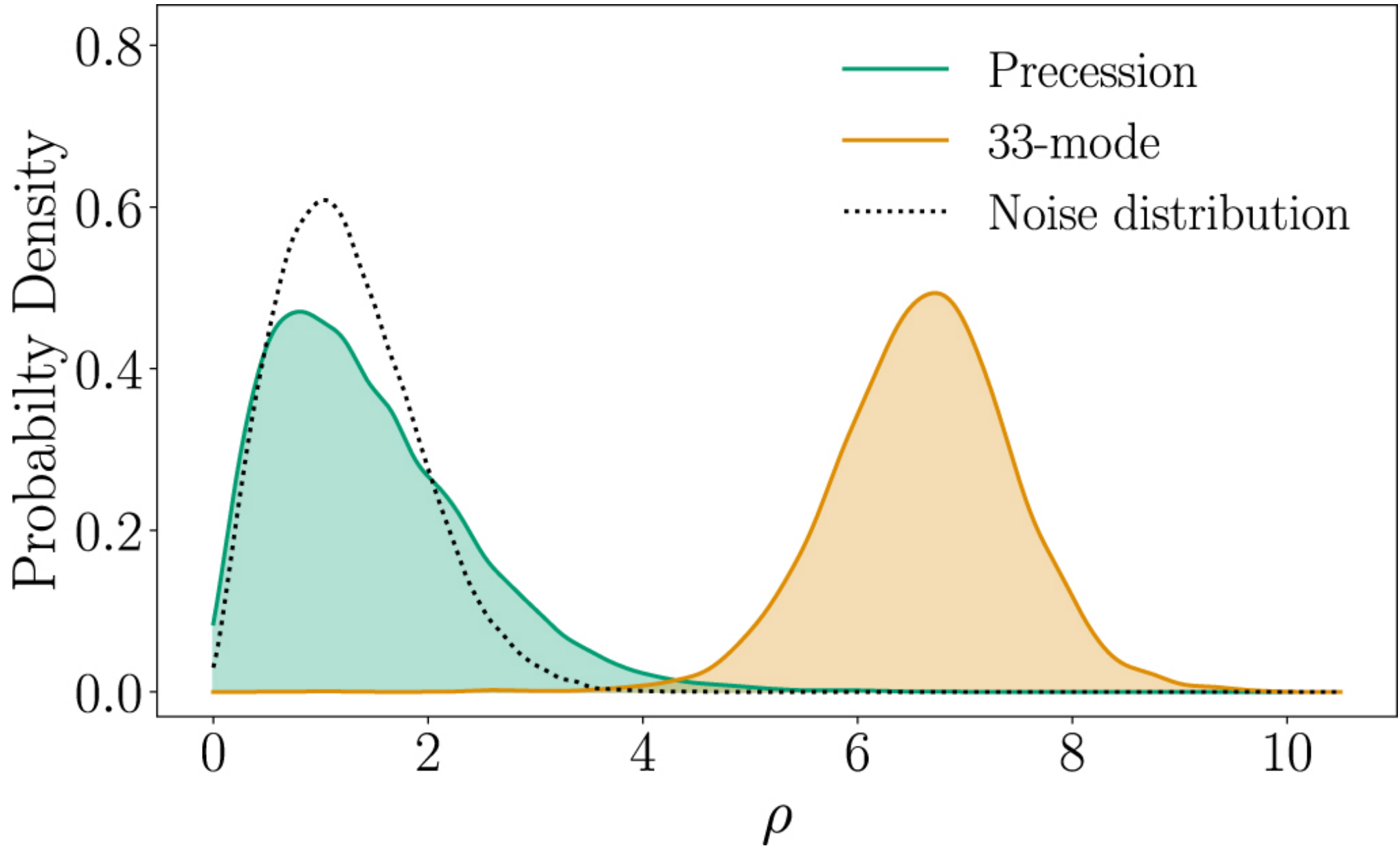
Figure 5. from GW190814: Gravitational Waves from the Coalescence of a 23 Solar Mass Black Hole with a 2.6 Solar Mass Compact Object null 2020 APJL 896 L44 doi:10.3847/2041-8213/ab960f https://dx.doi.org/10.3847/2041-8213/ab960f © 2020. The American Astronomical Society.
