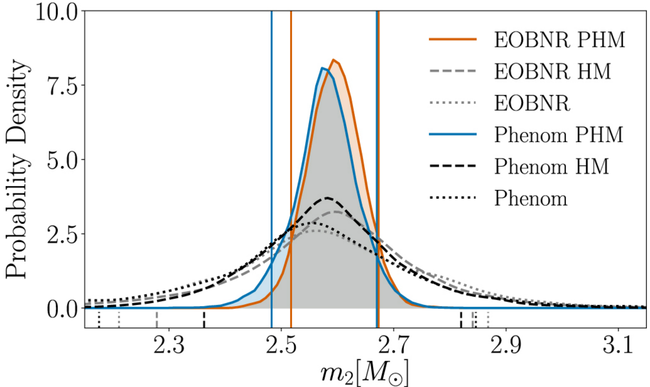
Figure 4. from GW190814: Gravitational Waves from the Coalescence of a 23 Solar Mass Black Hole with a 2.6 Solar Mass Compact Object null 2020 APJL 896 L44 doi:10.3847/2041-8213/ab960f https://dx.doi.org/10.3847/2041-8213/ab960f © 2020. The American Astronomical Society.
