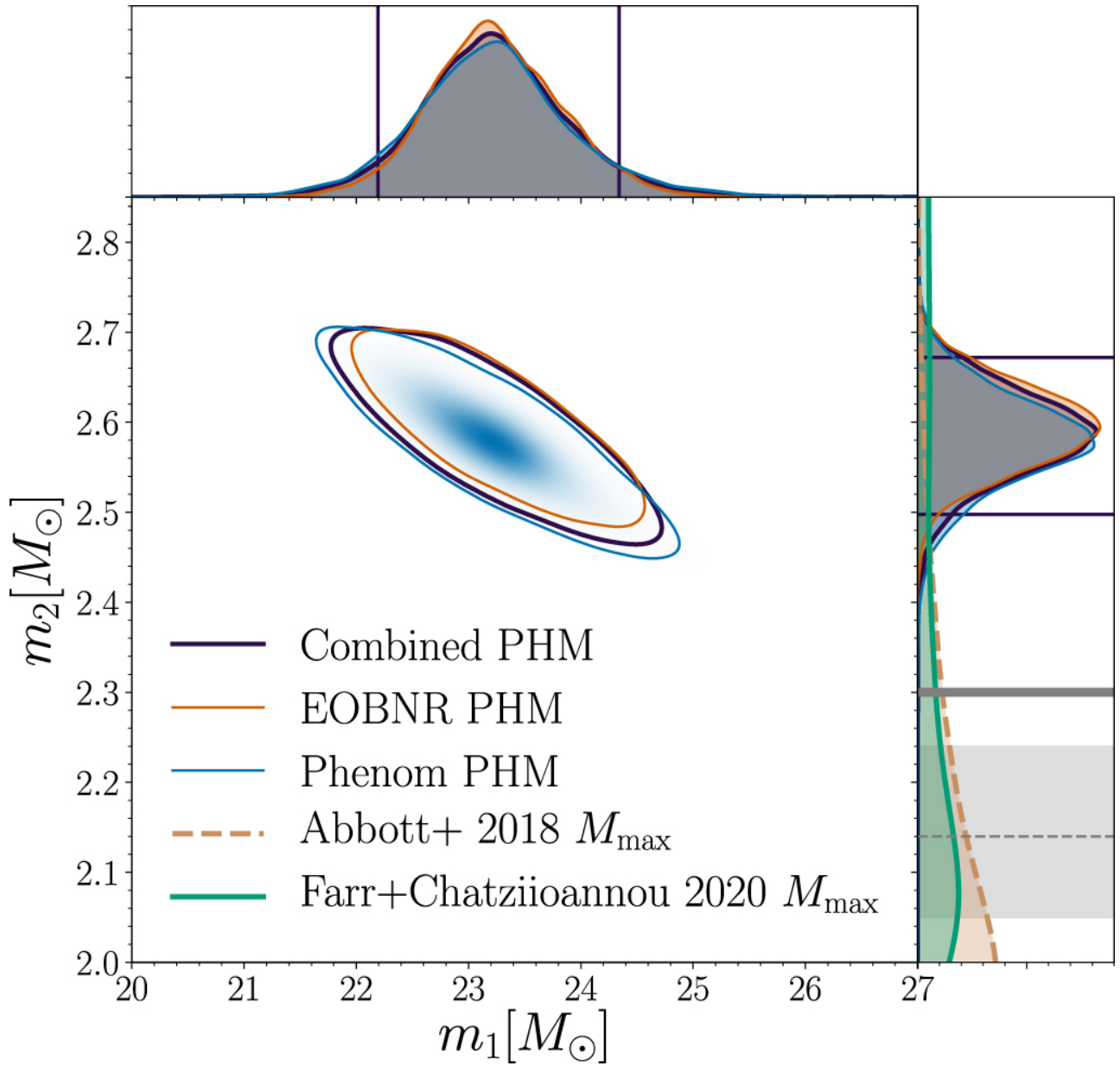
Figure 3. from GW190814: Gravitational Waves from the Coalescence of a 23 Solar Mass Black Hole with a 2.6 Solar Mass Compact Object null 2020 APJL 896 L44 doi:10.3847/2041-8213/ab960f https://dx.doi.org/10.3847/2041-8213/ab960f © 2020. The American Astronomical Society.
