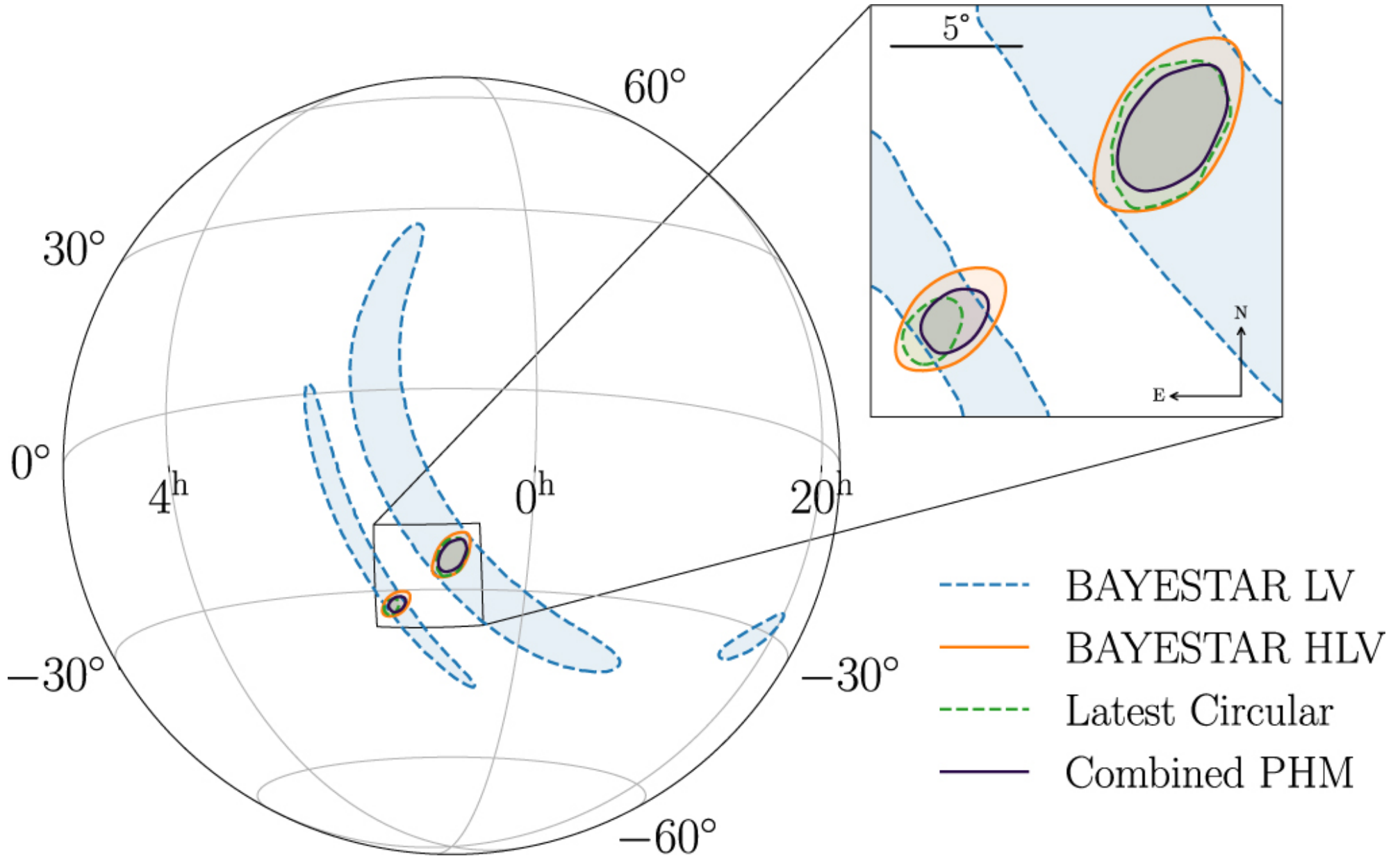
Figure 2. from GW190814: Gravitational Waves from the Coalescence of a 23 Solar Mass Black Hole with a 2.6 Solar Mass Compact Object null 2020 APJL 896 L44 doi:10.3847/2041-8213/ab960f https://dx.doi.org/10.3847/2041-8213/ab960f © 2020. The American Astronomical Society.
