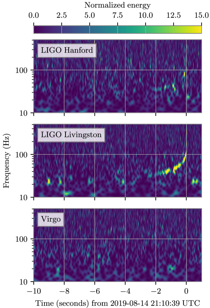
Figure 1. from GW190814: Gravitational Waves from the Coalescence of a 23 Solar Mass Black Hole with a 2.6 Solar Mass Compact Object null 2020 APJL 896 L44 doi:10.3847/2041-8213/ab960f https://dx.doi.org/10.3847/2041-8213/ab960f © 2020. The American Astronomical Society.
