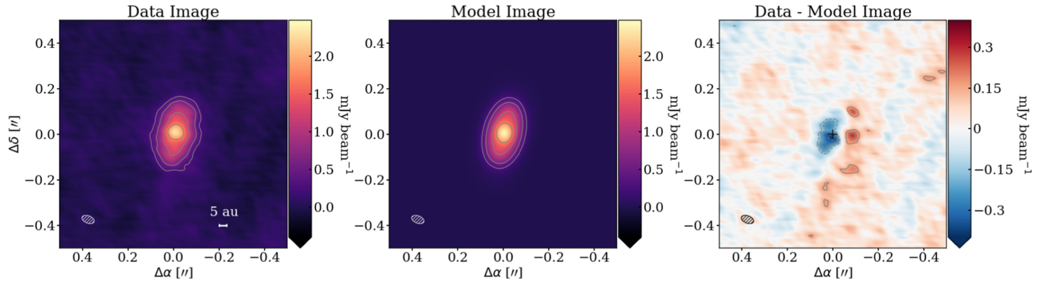
Figure 3. from Hints of a Population of Solar System Analog Planets from ALMA null 2020 APJL 895 L46 doi:10.3847/2041-8213/ab94a8 https://dx.doi.org/10.3847/2041-8213/ab94a8 © 2020. The American Astronomical Society. All rights reserved.
