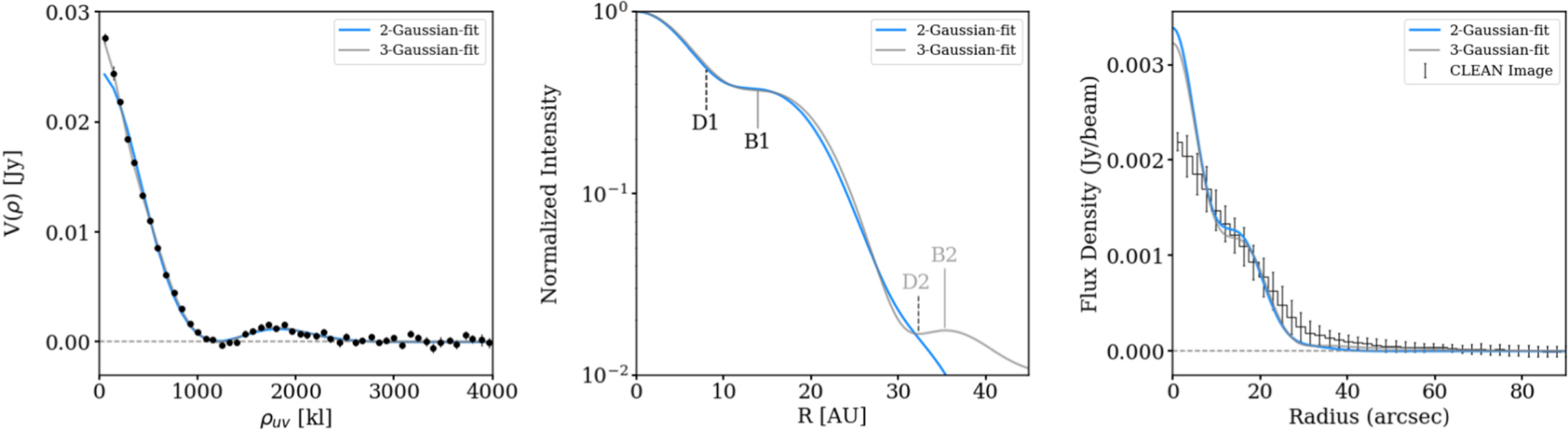
Figure 2. from Hints of a Population of Solar System Analog Planets from ALMA null 2020 APJL 895 L46 doi:10.3847/2041-8213/ab94a8 https://dx.doi.org/10.3847/2041-8213/ab94a8 © 2020. The American Astronomical Society. All rights reserved.
