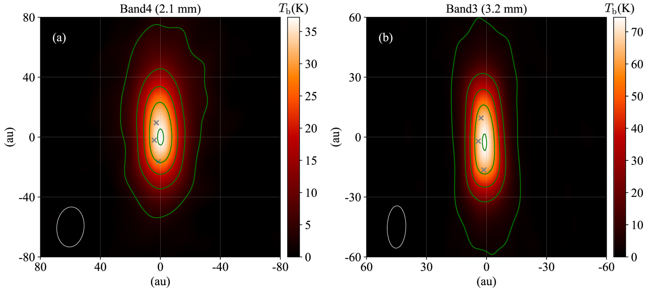
Figure A1. from Substructure Formation in a Protostellar Disk of L1527 IRS null 2020 APJL 895 L2 doi:10.3847/2041-8213/ab8eaa https://dx.doi.org/10.3847/2041-8213/ab8eaa © 2020. The American Astronomical Society. All rights reserved.
