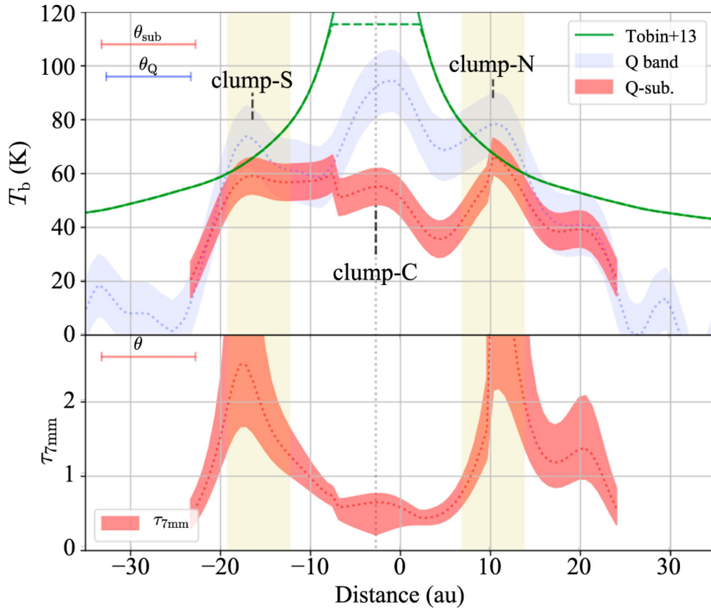
Figure 3. from Substructure Formation in a Protostellar Disk of L1527 IRS null 2020 APJL 895 L2 doi:10.3847/2041-8213/ab8eaa https://dx.doi.org/10.3847/2041-8213/ab8eaa © 2020. The American Astronomical Society. All rights reserved.
