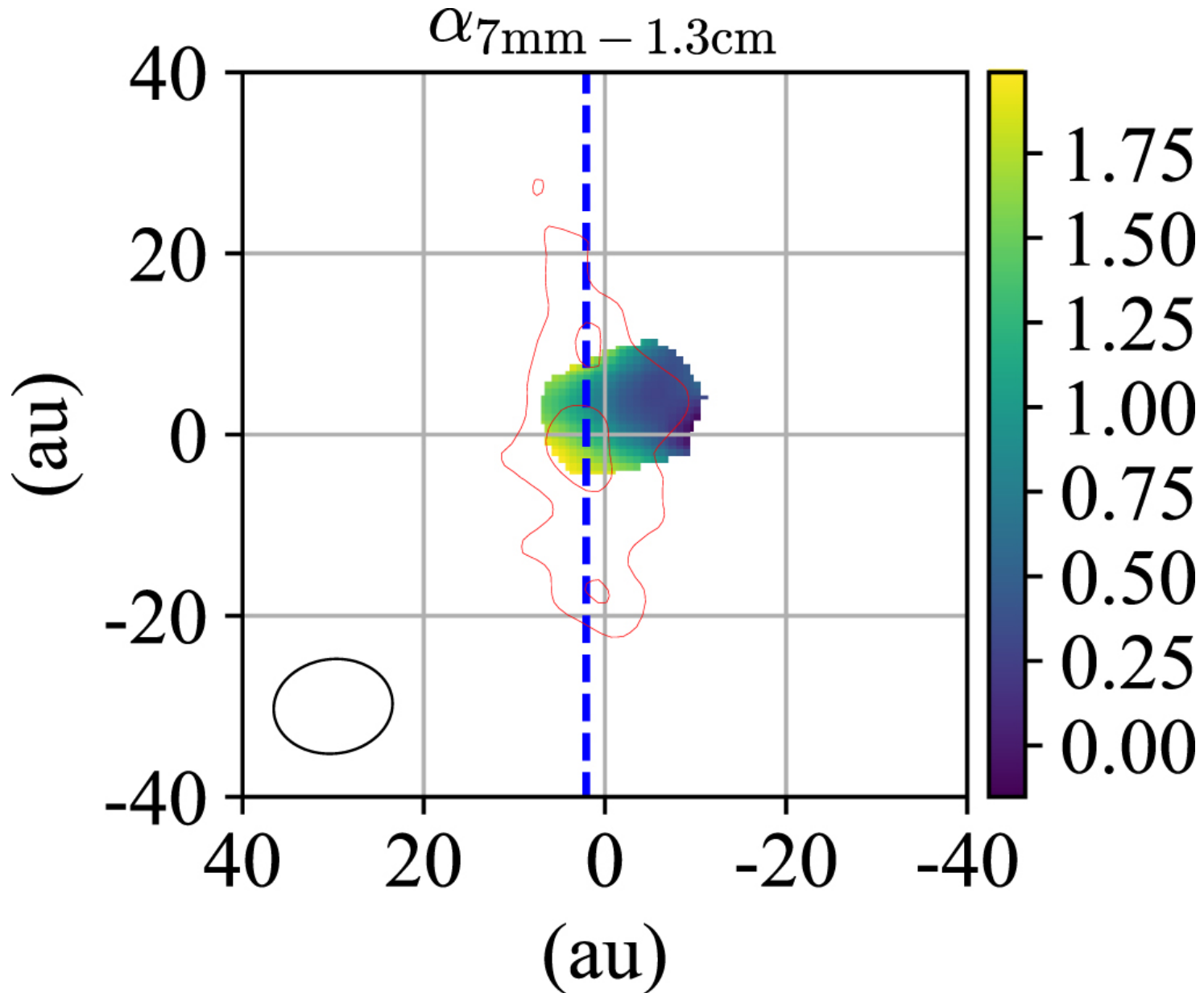
Figure 2. from Substructure Formation in a Protostellar Disk of L1527 IRS null 2020 APJL 895 L2 doi:10.3847/2041-8213/ab8eaa https://dx.doi.org/10.3847/2041-8213/ab8eaa © 2020. The American Astronomical Society. All rights reserved.
