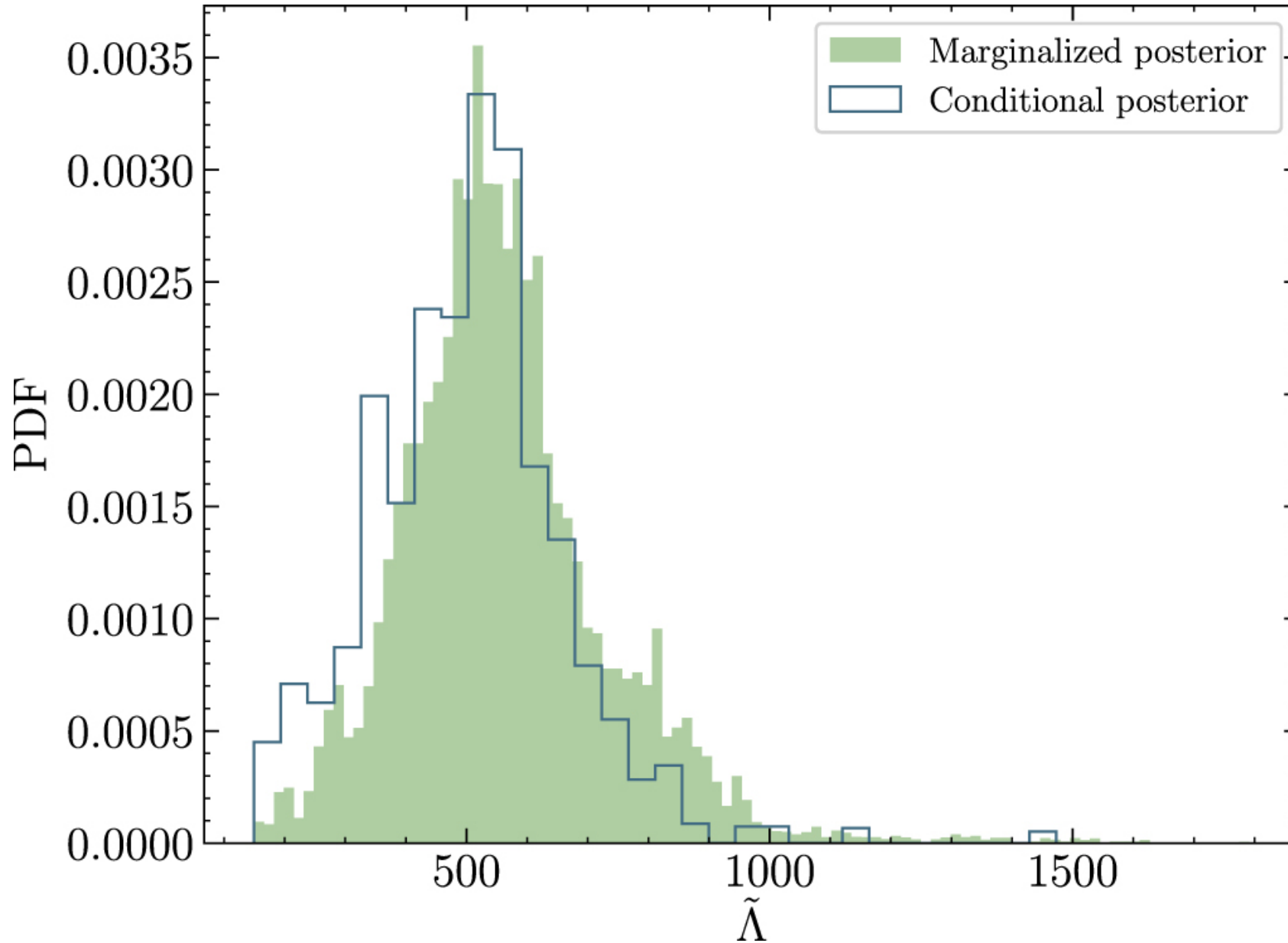
Figure B2. from Constraining the Dense Matter Equation of State with Joint Analysis of NICER and LIGO/Virgo Measurements null 2020 APJL 893 L21 doi:10.3847/2041-8213/ab822f https://dx.doi.org/10.3847/2041-8213/ab822f © 2020. The American Astronomical Society. All rights reserved.
