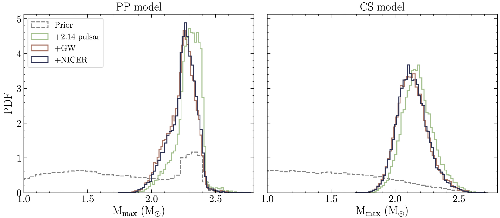
Figure 6. from Constraining the Dense Matter Equation of State with Joint Analysis of NICER and LIGO/Virgo Measurements null 2020 APJL 893 L21 doi:10.3847/2041-8213/ab822f https://dx.doi.org/10.3847/2041-8213/ab822f © 2020. The American Astronomical Society. All rights reserved.
