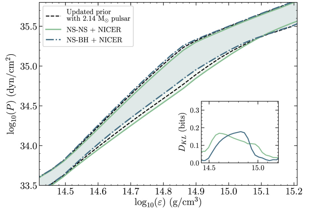
Figure 5. from Constraining the Dense Matter Equation of State with Joint Analysis of NICER and LIGO/Virgo Measurements null 2020 APJL 893 L21 doi:10.3847/2041-8213/ab822f https://dx.doi.org/10.3847/2041-8213/ab822f © 2020. The American Astronomical Society. All rights reserved.
