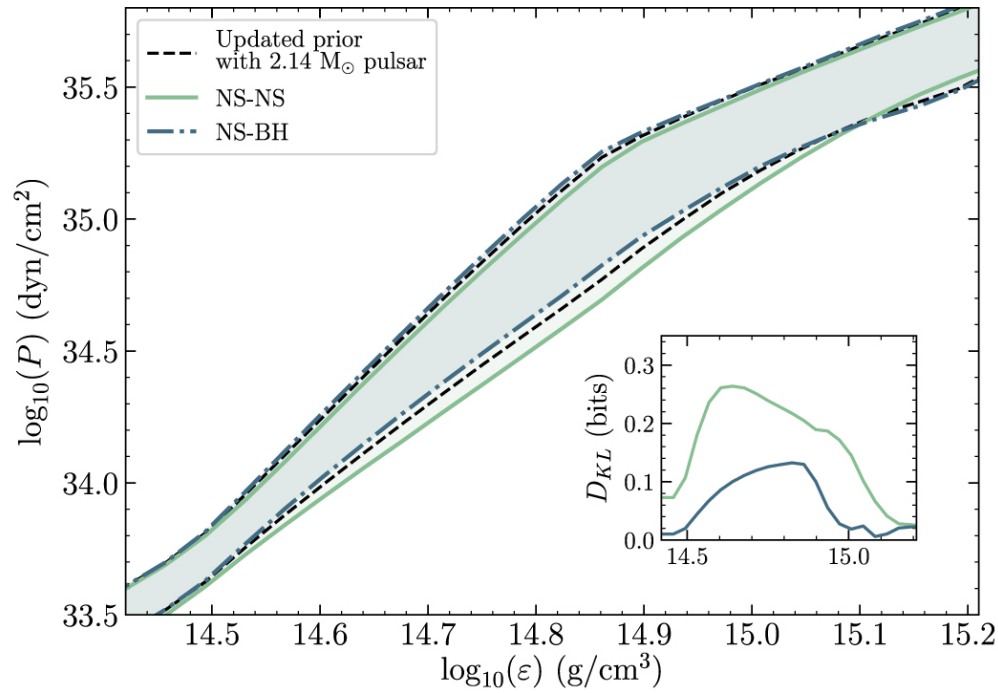
Figure 5. from Constraining the Dense Matter Equation of State with Joint Analysis of NICER and LIGO/Virgo Measurements null 2020 APJL 893 L21 doi:10.3847/2041-8213/ab822f https://dx.doi.org/10.3847/2041-8213/ab822f © 2020. The American Astronomical Society. All rights reserved.
