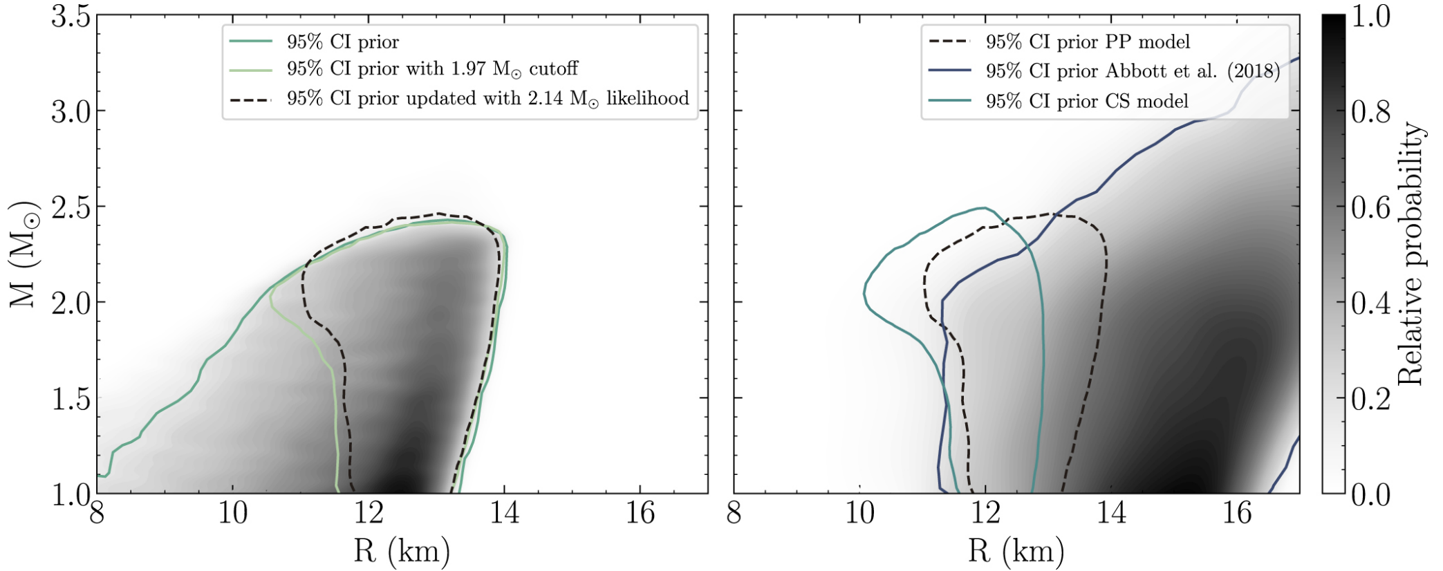
Figure 2. from Constraining the Dense Matter Equation of State with Joint Analysis of NICER and LIGO/Virgo Measurements null 2020 APJL 893 L21 doi:10.3847/2041-8213/ab822f https://dx.doi.org/10.3847/2041-8213/ab822f
