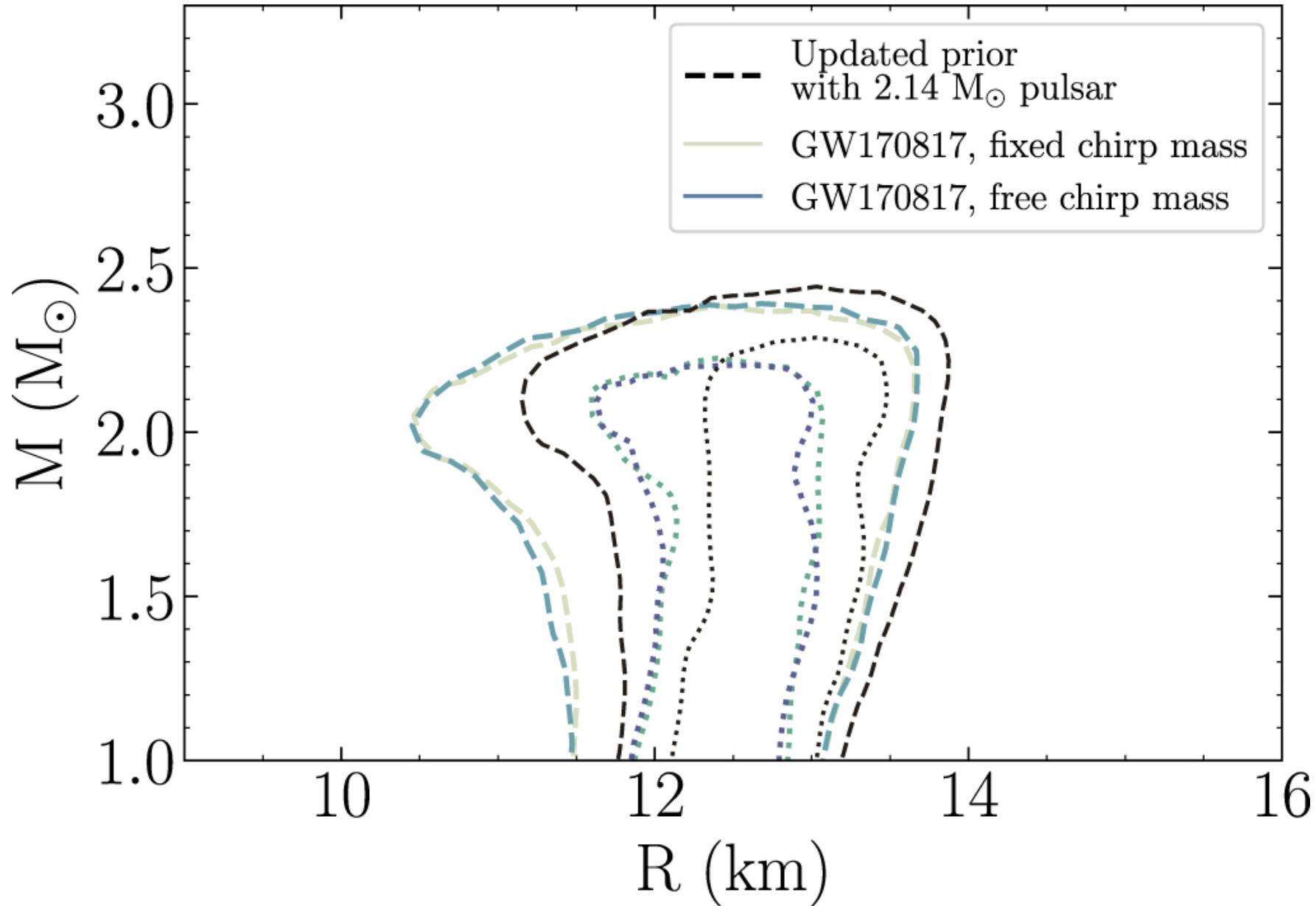
Figure 1. from Constraining the Dense Matter Equation of State with Joint Analysis of NICER and LIGO/Virgo Measurements null 2020 APJL 893 L21 doi:10.3847/2041-8213/ab822f https://dx.doi.org/10.3847/2041-8213/ab822f © 2020. The American Astronomical Society. All rights reserved.
