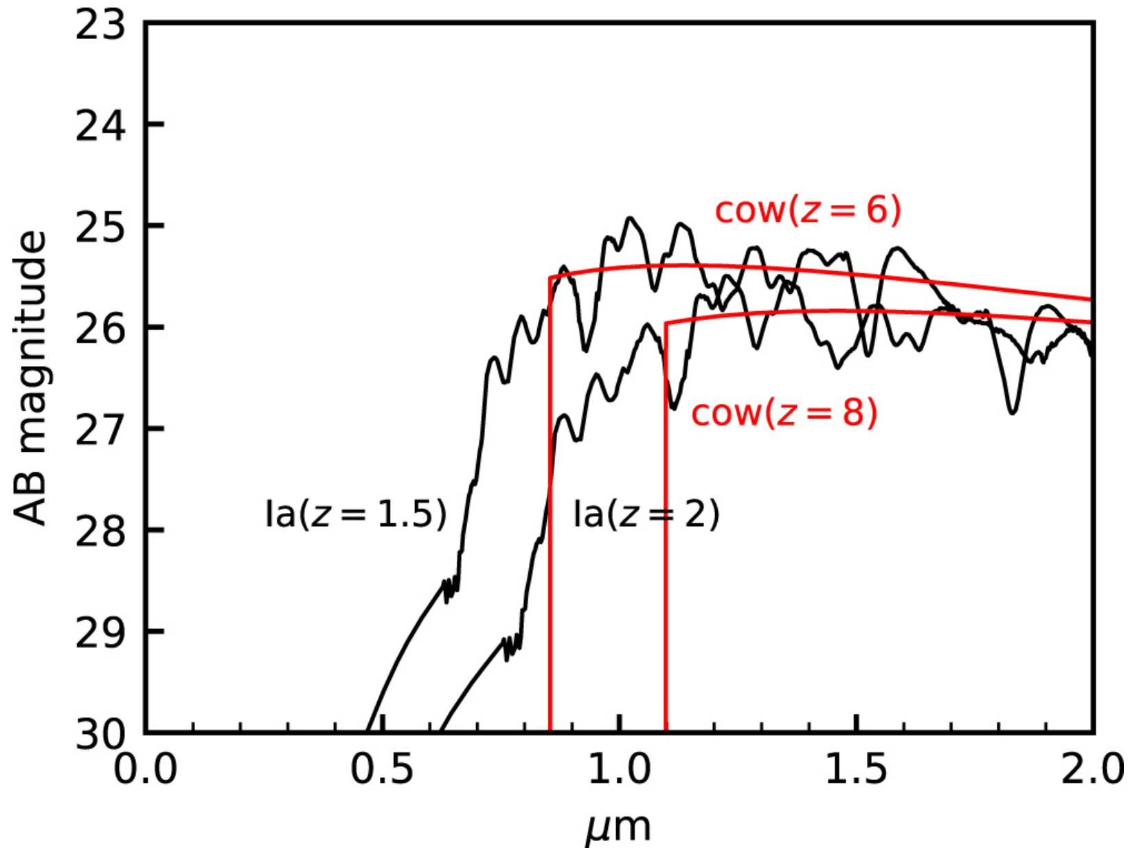
Figure 5. from Fast Luminous Blue Transients in the Reionization Era and Beyond null 2020 APJL 890 L17 doi:10.3847/2041-8213/ab7240 https://dx.doi.org/10.3847/2041-8213/ab7240 © 2020. The American Astronomical Society. All rights reserved.
