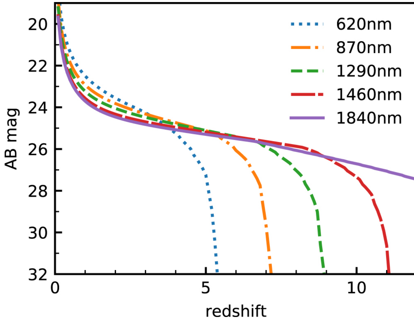
Figure 2. from Fast Luminous Blue Transients in the Reionization Era and Beyond null 2020 APJL 890 L17 doi:10.3847/2041-8213/ab7240 https://dx.doi.org/10.3847/2041-8213/ab7240 © 2020. The American Astronomical Society. All rights reserved.
